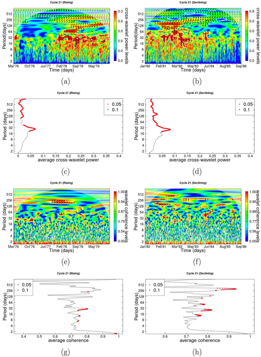
Figure 3. (a), (b) XWT power plots of GMI (ap-index) and SSN ( R_z ) of solar cycle 21, depicting interaction and phase behavior (marked by arrows) of Sun's activity vis-a-vis geomagnetic disturbances caused. (c), (d) Average cross-wavelet power plots showing average power value vs. periods of R_z and ap-index for solar cycle 21. The red-dots on the curve confirm 95% confidence level in the estimation. (e), (f) Wavelet coherence power plots of the Sun's activity ( R_z ) varying with geomagnetic disturbances (ap-index) of solar cycle 21, exhibiting significant phase mixing (marked by randomly oriented arrows) in case of 27 day period, as is also evident from (a) and (b), across time duration considered. (g), (h) Average coherence power plot of R_z and ap-index for solar cycle 21, displaying significant coherence value of all estimated periodic interactions of the two time series.
