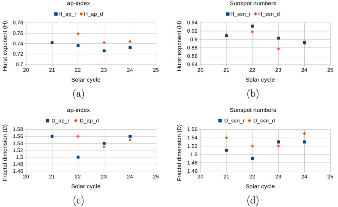
Figure 5. Results obtained: (a) Hurst exponent ( H ) estimated for ap-index during rising ( r ) and declining ( d ) phases over all the four solar cycles considered, (b) H estimated for SSNs, (c) fractal dimension ( D ) estimated for ap-index, and (d) D estimated for SSN.
