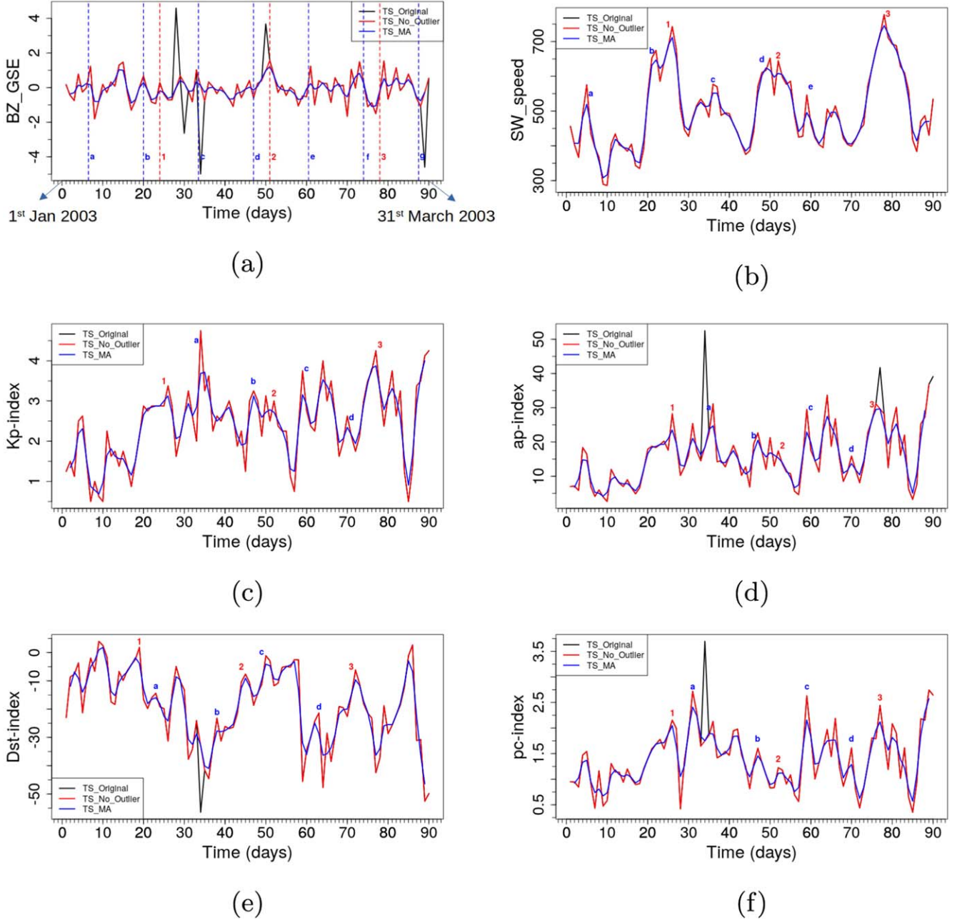
Figure 1. Plots of IMF, SW and GMI time series for 90 days during the declining phase of solar cycle 23 (ranging from 2003 January 1 to March 31), along with the MA, and cleaned (without the outliers) series. The 13.5 day ( a - b \approx b - c \approx c - d \approx d - e \approx e - f \approx f - g \approx 13.5 day) and 27 day ( 1 - 2 \approx 2 - 3 \approx 27 day) periods are observed in all the time series.
