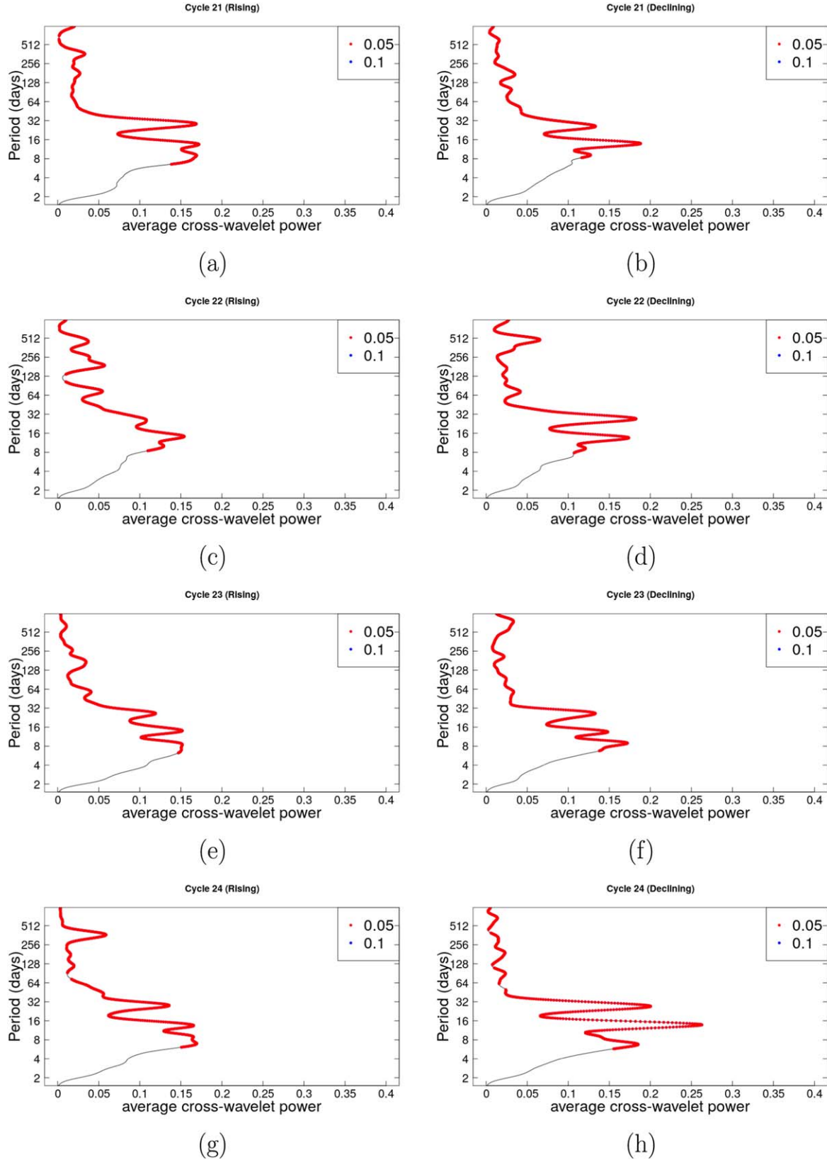
Figure 4. Average cross-wavelet power plots of SW plasma speed and GMI (ap-index).
