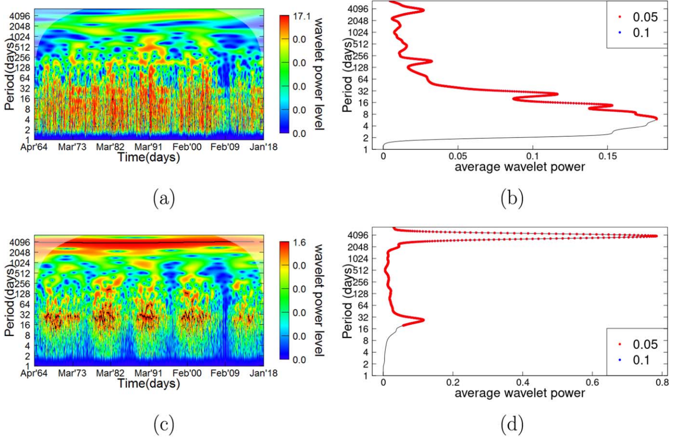
Figure 6. (a) Continuous wavelet power of ap-index (GMI) for five solar cycles, (b) average wavelet plot of ap-index, (c) continuous wavelet power of SSN for five solar cycles and (d) average wavelet plot of SSN.
