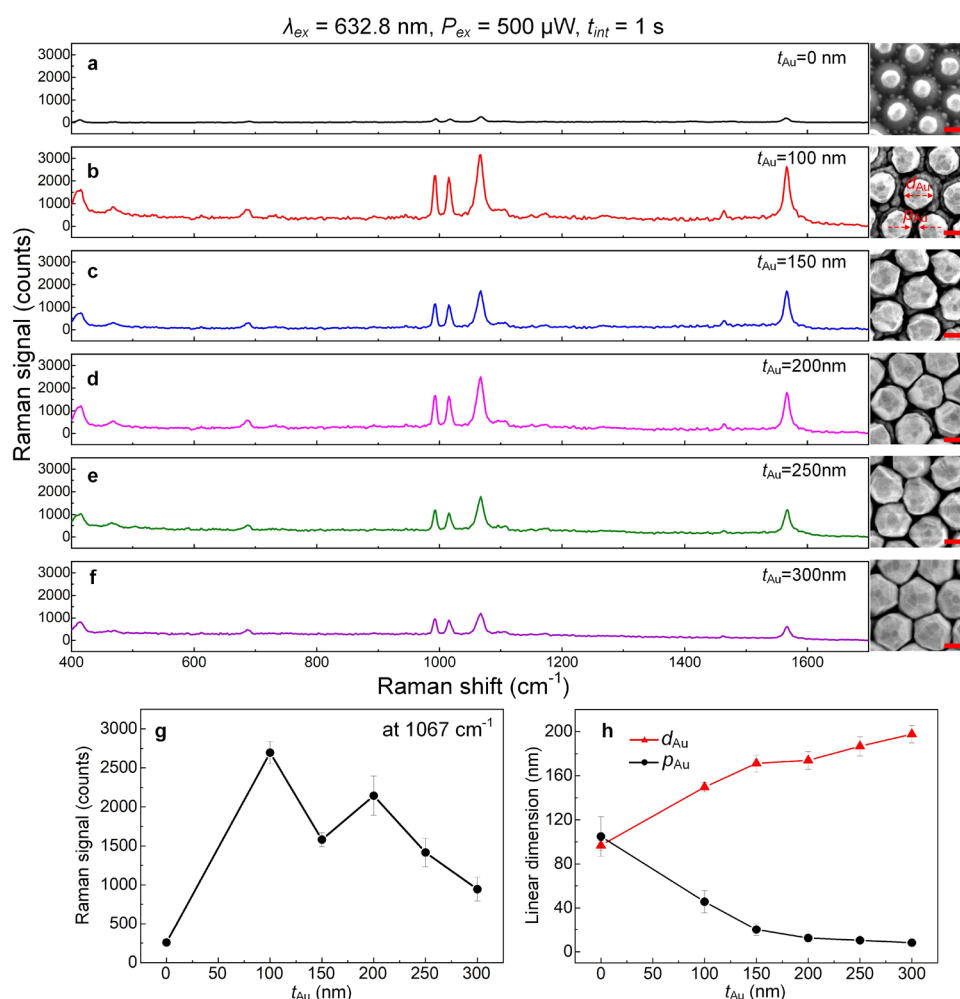
Figure 6. Close-up HR-SEM images (scale bars: 100 nm) of \text{Au}_{15\text{ s}}^{200\text{ W}} \text{d}_{\text{SiO}_2}^{200\text{ nm}} @ \text{PPMs} covered with an Au film of different thicknesses ( t_{Au} ) (a) 0, (b) 100, (c) 150, (d) 200, (e) 250, and (f) 300 nm and their corresponding Raman spectra. (g) Raman signal at 1067 cm -1 as a function of t_{Au} . The error bars were obtained from 10 spectra captured randomly on different microspheres and different locations on each microsphere. (h) d_{Au} and p_{Au} as a function of t_{Au} , obtained by measuring 20 different diameters and nanogap distances on a single microsphere. Error bars in panels (g) and (h) represent the standard deviation.
