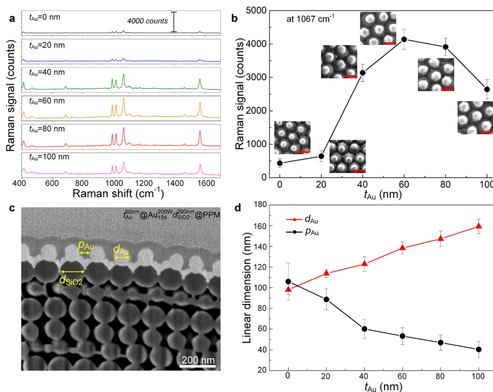
Figure 7. Au-coated PPMs with different t_{Au} values. (a) Raman spectra and (b) their corresponding Raman intensity at 1067 cm -1 as a function of t_{Au} . The error bars were obtained from 10 spectra captured randomly on different microspheres and different locations per microsphere. Insets are the corresponding HR-SEM top-view images. Scale bar: 200 nm. (c) Cross-sectional HR-SEM images of Au-coated PPMs ( t_{Au}^{60\text{ nm}}@Au_{15\text{ s}}^{200\text{ W}}d_{SiO2}^{200\text{ nm}}@PPM ). (d) d_{Au} and p_{Au} as a function of t_{Au} obtained by measuring 20 different diameters and nanogap distances on a single microsphere. Error bars in panels (b) and (d) indicate the standard deviation.
