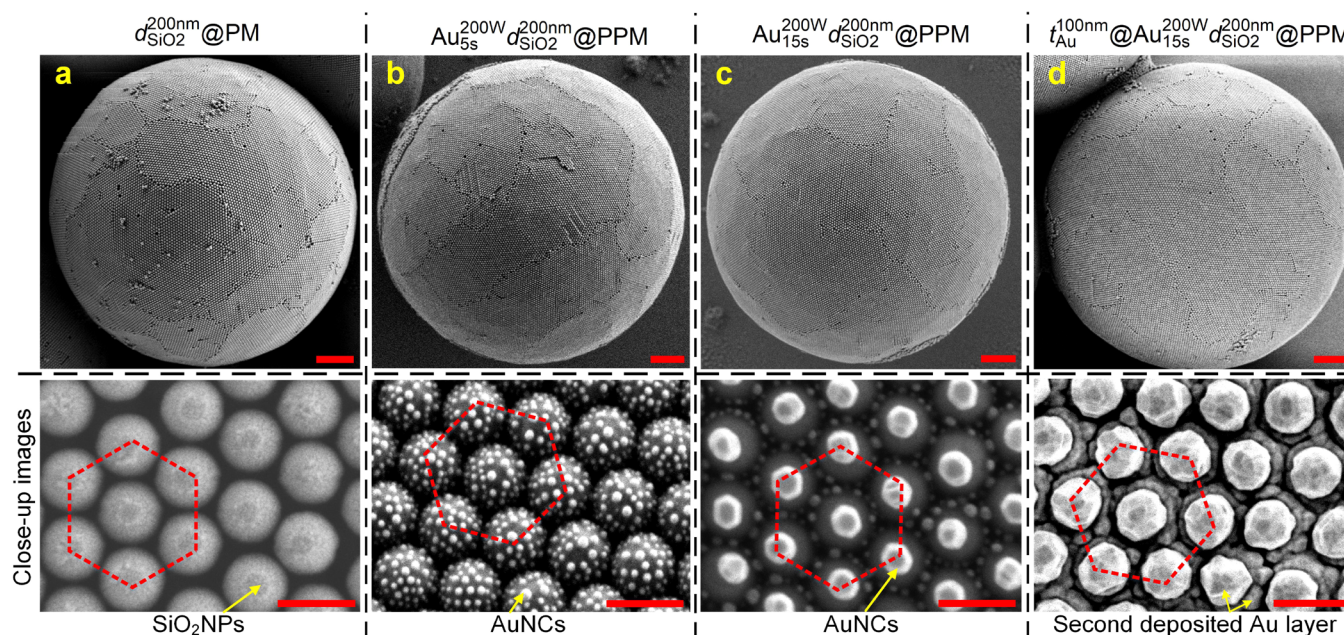
Figure 2. Top-view HR-SEM images (scale bar: 2 \mu\text{m} ) of (a) a d_{\text{SiO}_2}^{200\text{nm}} @ \text{PM} , (b) a \text{Au}_{5\text{s}}^{200\text{W}} d_{\text{SiO}_2}^{200\text{nm}} @ \text{PPM} , (c) a \text{Au}_{15\text{s}}^{200\text{W}} d_{\text{SiO}_2}^{200\text{nm}} @ \text{PPM} , and (d) a t_{\text{Au}}^{100\text{nm}} @ \text{Au}_{15\text{s}}^{200\text{W}} d_{\text{SiO}_2}^{200\text{nm}} @ \text{PPM} and close-up images (scale bar: 200 nm) of their corresponding surface morphologies.
