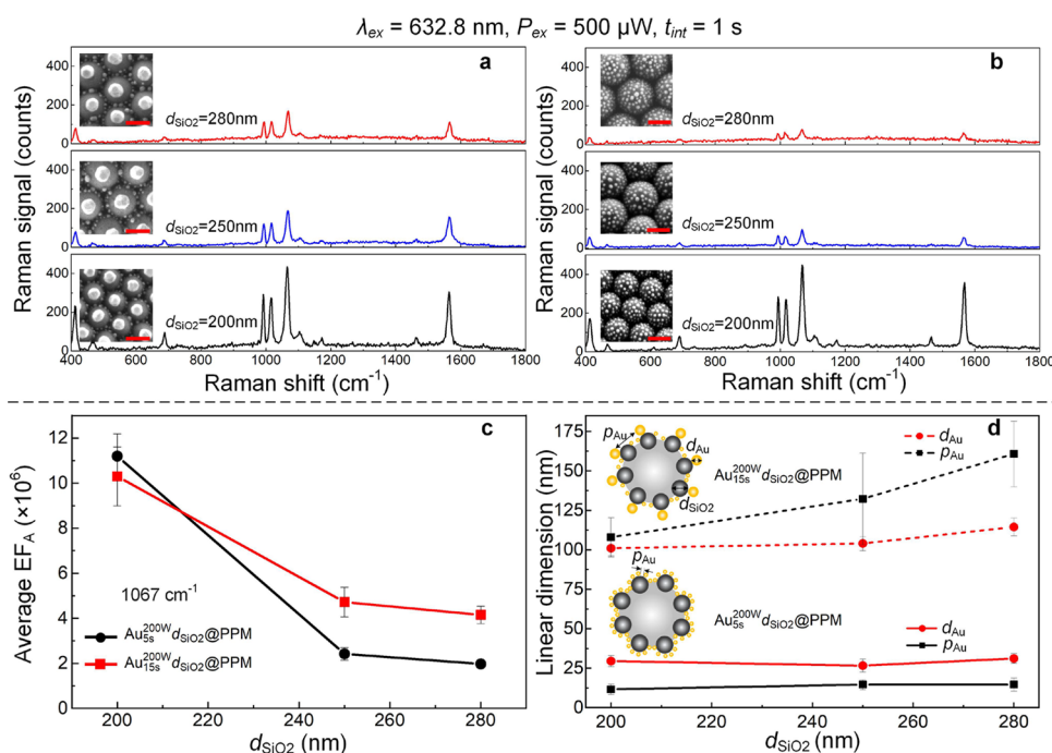
Figure 5. Raman spectra of various PPMs featuring (a) one large AuNC and (b) multiple small AuNCs on top of each \text{SiO}_2 NP and their corresponding top-view HR-SEM images (scale bars: 200 nm). (c) Average \text{EF}_A ( 1067 \text{ cm}^{-1} ) of PPMs as a function of the d_{\text{SiO}_2} . The error bars were obtained from 10 spectra captured randomly on different microspheres and different locations on each microsphere. (d) d_{\text{Au}} (diameter) and p_{\text{Au}} (gap) of the AuNCs as a function of the d_{\text{SiO}_2} , obtained by measuring 20 different diameters and nanogap distances on a single microsphere. Error bars in panels (c) and (d) represent the standard deviation.
