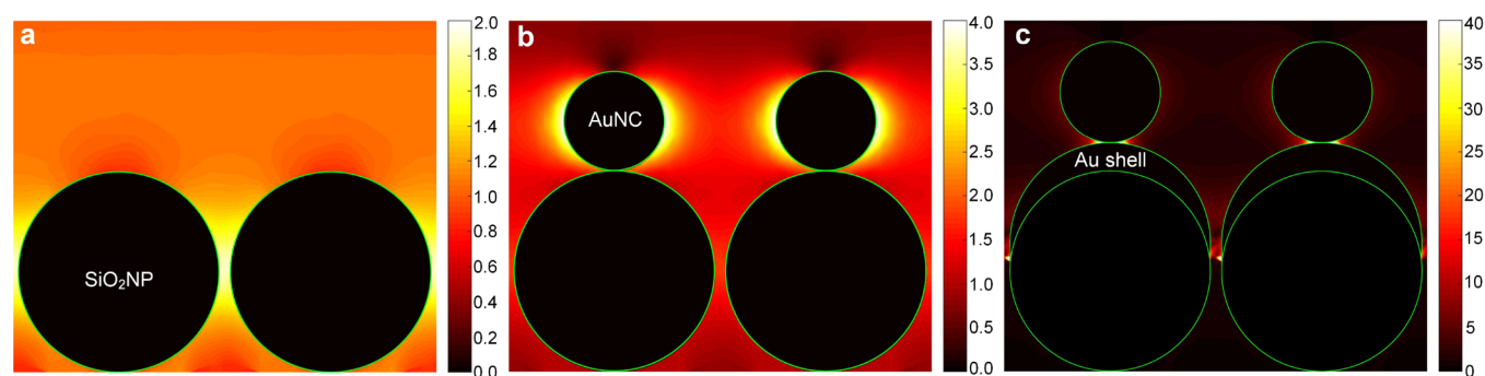
Figure 8. Cross sections of the simulated electric field distribution on different structures. The color bars represent |E|/|E_0| . (a) Pure PM, d_{\text{SiO}_2}^{200 \text{ nm}} @ \text{PM} . (b) PPM, \text{Au}_{15 \text{ s}}^{200 \text{ nm}} d_{\text{SiO}_2}^{200 \text{ nm}} @ \text{PPM} . (c) Au-coated PPM, t_{\text{Au}} @ \text{Au}_{15 \text{ s}}^{200 \text{ nm}} d_{\text{SiO}_2}^{200 \text{ nm}} @ \text{PPM} . (panels (a–c)) The diameter of constituent \text{SiO}_2\text{NP} is 200 nm, and the AuNC is 100 nm in diameter. Please note that in all figures, the spatial location that we show is on top of an extended PC structure consisting of 20 layers of a hexagonal lattice of \text{SiO}_2\text{NPs} . The periodicity of 210 nm is chosen. The green lines indicate the outline of the \text{SiO}_2\text{NPs} , AuNCs, and Au shells.
