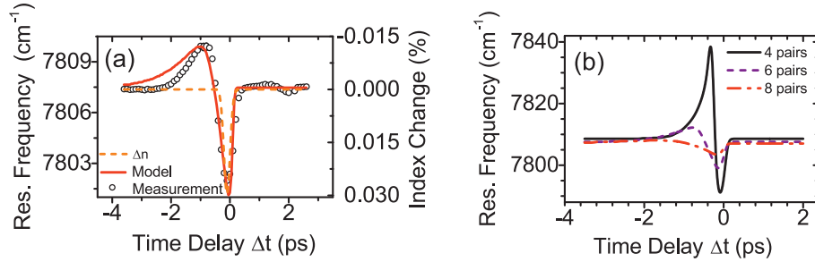
Fig. 2. (a) Measured (symbols) and calculated (red curve) resonance frequency versus time delay ( \Delta t ) between pump and probe for a GaAs/AlAs cavity ( Q = 390 \pm 60 ). The resonance frequency red-shifts due to increased refractive index only near temporal overlap ( \Delta t = 0 \pm 15 fs) of pump-probe, shown with dashed curve. (b) Calculated spectra for a GaAs/AlAs cavity that consists of 19 pairs of bottom Bragg layers, \lambda -layer, and sequentially changed number of layers on the top Bragg mirror.
