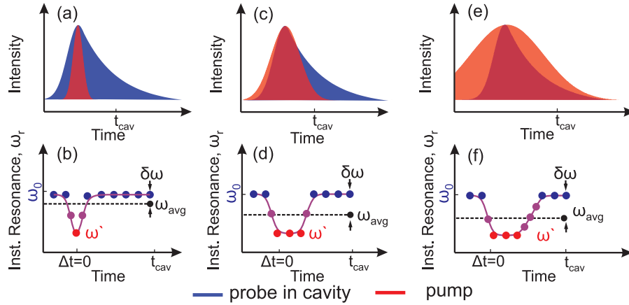
Fig. 8. Schematic representation of the pump and probe pulses in the cavity for three different pump pulse durations. The peak intensity of the pump pulse is kept constant while stretching the pump pulse. The lower panels show the instantaneous frequency shift versus time. The cavity resonance instantaneously shifts from \omega_0 to \omega' at pump probe overlap ( \Delta t = 0 ). The detected resonance shift ( \omega_{avg} ) is deduced from the transient reflectivity that is a result of the time averaging of the cavity storage and detector response time.
