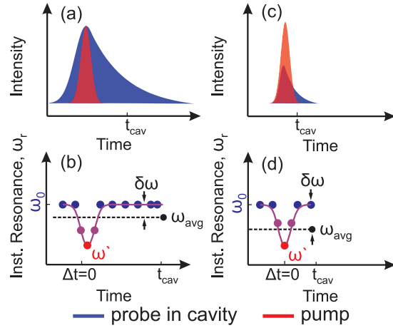
Fig. 6. Schematic representation of the pump and probe pulses in the cavity for two different quality factor cavities, (a) high- Q , (c) low- Q . The lower panels show the instantaneous frequency shift versus time. The cavity resonance instantaneously shifts from \omega_0 to \omega' at pump probe overlap ( \Delta t = 0 ). The detected resonance shift ( \omega_{avg} ) is deduced from the transient reflectivity that is a result of the time averaging of the cavity storage and detector response time. A larger resonance frequency shift \delta\omega is observed for cavities with shorter storage times.
