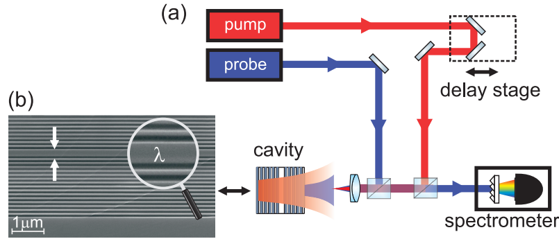
Fig. 1. (a) Schematic of the all-optical switch setup. The probe beam path is shown in blue, the pump beam path in red. The time delay between pump and probe pulses is set with a delay stage. The reflected signal from the cavity is spectrally resolved and detected. (b) SEM picture of the multilayer structure of a GaAs/AlAs microcavity. GaAs layers appear light grey, and AlAs layers dark grey. The white arrows indicate the thickness of the GaAs \lambda -layer. The GaAs substrate is seen at the bottom. The magnifier shows a more detailed view on how the \lambda -layer is sandwiched between the Bragg stacks.
