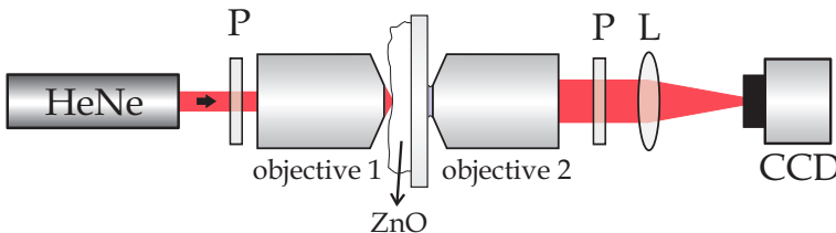
Figure 7.1.: Experimental setup. HeNe: laser. ZnO: sample. Objective 1: 100× 0.9-NA objective. Objective 2: 100× 1.3-NA oil immersion objective. L: 200 mm focal length lens. P: polarizer. CCD: camera sensor.
