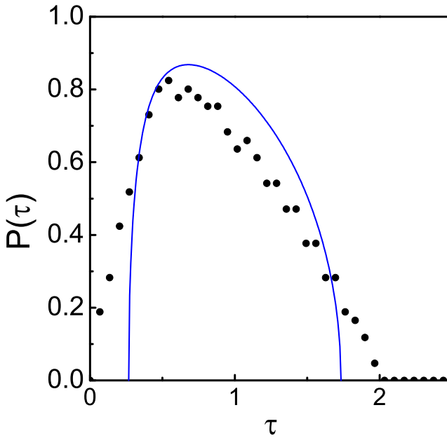
Figure 5.14.: Black dots: Normalized singular value histogram of the transmission matrix of the thin sample, normalized by \sqrt{\langle \tau^2 \rangle} . Solid curve: Marcenko-Pastur density, with \gamma = 1.86 .
