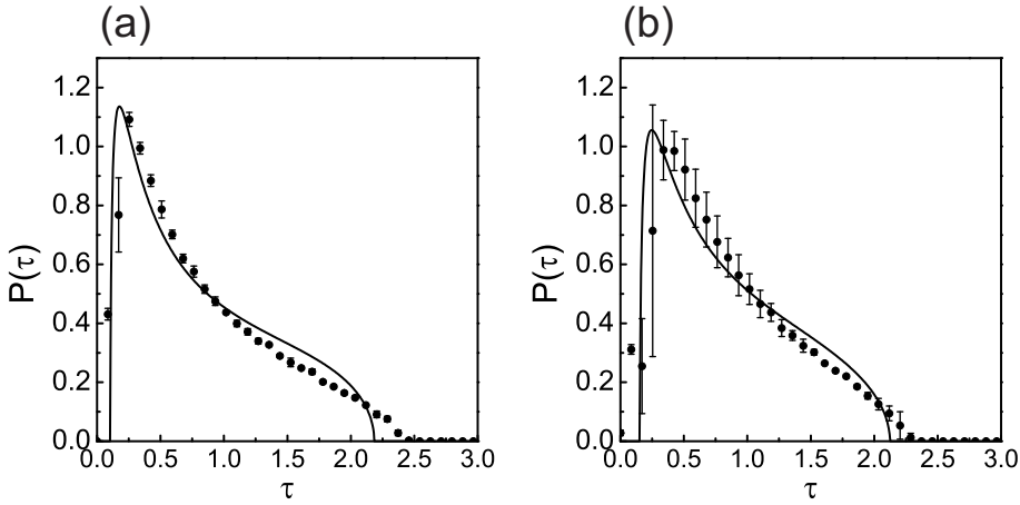
Figure 6.10.: Singular value densities obtained from the analytical model and the experiment for (a) thin (b) thick sample with dense sampling of incident fields (normalization factor = \sqrt{\langle \tau^2 \rangle} ). Black dots: mean, black errorbars: standard deviation of the normalized bin counts in 3 experimental singular value histograms. Solid curve: Histogram obtained from analytical model using n_{\text{eff}} = 1.4 and l_{\text{tr}} = 0.63 \mu\text{m} , with no adjusted parameters.
