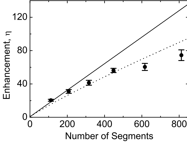
Figure 3.4.: Intensity enhancement at the target position versus the number of segments on the SLM. Black solid line: enhancements expected under ideal conditions, as obtained from Eq. 3.3. Each data point (black circles) is an ensemble average of 14-25 data points obtained from measurements. Bars represent the standard error of each measurement set. Black dotted curve: fit performed for the experimental enhancements using Eq. 3.4 with a single free parameter, SNR. Best curve fit yields SNR=24.
