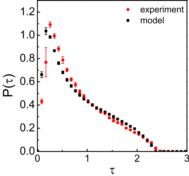
Figure 6.8.: Normalized singular value histograms obtained from the experiment and from the model using l_{tr} = 0.65 \mu\text{m} and n_{\text{eff}} = 1.4 , with normalization factor, \sqrt{\langle \tau^2 \rangle} . Red dots: mean, red errorbars: standard deviation of 3 experimental singular value histograms. Black squares: mean, black errorbars: standard deviation of singular value histograms obtained from 20 runs of the model.
