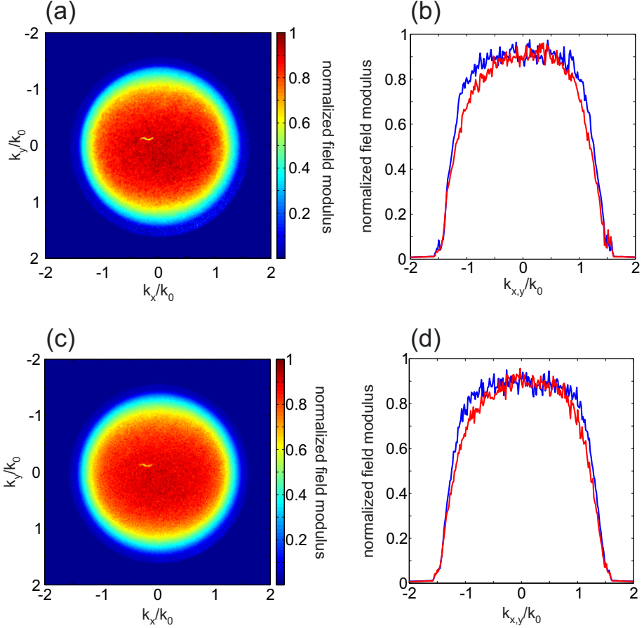
Figure 6.2.: (a, c) Momentum-space density map of root mean square fields, \sqrt{\langle |E(k)|^2 \rangle} transmitted through the 11- \mu\text{m} and 30- \mu\text{m} thick layer of ZnO nanoparticles on glass. (b, d) Cross sections of the images in (a, c) along x- (blue curve) and y- (red curve) directions. The illumination NA is 0.95.
