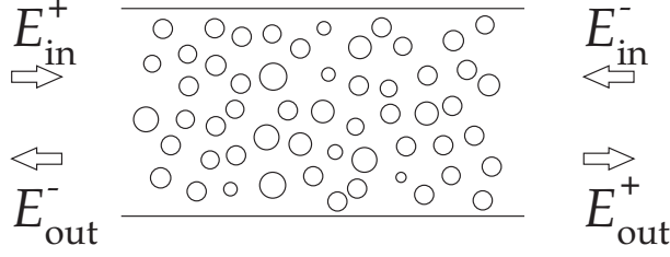
Figure 2.2.: E_{in}^+ : field incident on the sample from the left, E_{out}^+ : field transmitted through the sample on the right, E_{in}^- : field incident on the sample from the right. E_{out}^- : field transmitted through the sample on the left.
