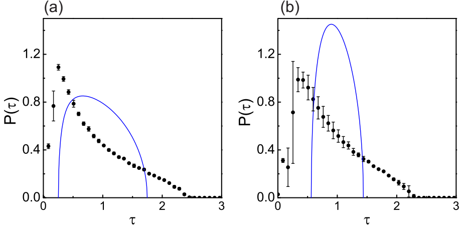
Figure 6.7.: Normalized singular value histograms of the transmission matrix of (a) thin sample, (b) thick sample in the case of dense sampling, normalization factor =\sqrt{\langle\tau^2\rangle} . Black dots: mean, errorbars: standard deviation of the normalized counts in the singular value histograms of three different transmission matrices. Solid curve: Marcenko-Pastur singular value density with (a) \gamma = 1.79 , (b) \gamma = 5.2 .
