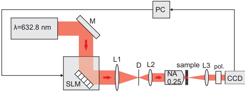
Figure 3.5.: Experimental setup for MEMS-based focusing. A HeNe laser beam that has a wavelength of 632.8 nm and output power of 2 mW is expanded and used to illuminate the SLM via a mirror (M). L1, L2 and L3 are planoconvex lenses with respectively 150 mm, 50 mm and 50 mm focal lengths. D is an aperture used for spatial filtering, and NA 0.25 is a microscope objective having 10 \times magnification and 0.25 numerical aperture. Light exiting the sample is converted to far field with L3, passed through a polarizer, pol. and projected on a CCD camera, which is connected to the SLM via a PC.
