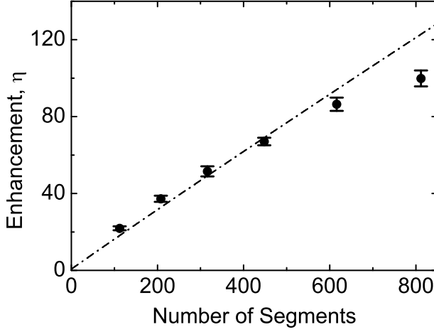
Figure 3.7.: Numerically simulated intensity enhancement at the target position versus the number of segments that the SLM is divided into. Each data point represented by the black circles is an ensemble average of a set of data points obtained from simulations conducted with an intensity noise of SNR=165 . Bars represent the standard error of each measurement set. The dashed line shows the enhancements obtained from Eq. 3.25, assuming \langle A \rangle^2 / \langle A^2 \rangle = 1 and using Eq. 3.19.
