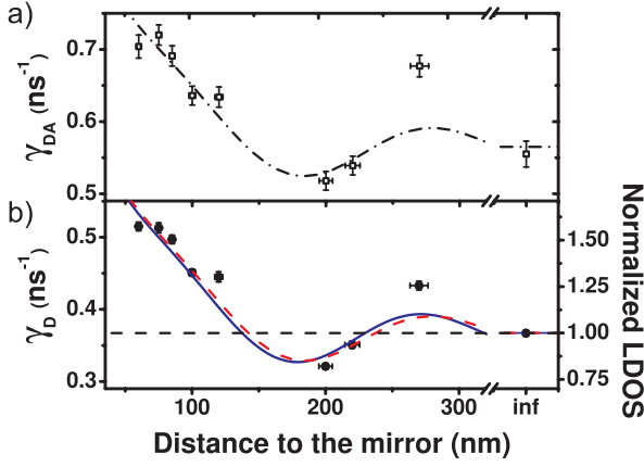
FIG. 2 (color). (a) Total donor decay rate \gamma_{DA} of the FRET samples oscillates with distance to the mirror. Dash-dotted curve: model consisting of the calculated LDOS, averaged over the whole donor emission band, plus a constant FRET rate \gamma_{\text{FRET}} = 0.197 \pm 0.006 \text{ ns}^{-1} . (b) The total decay rate \gamma_D of the donor-only samples shows the well-known oscillation as a function of distance d to the mirror. Solid blue curve: calculated LDOS for the center of the detection band at 525 nm; dashed red: calculated LDOS, averaged over the whole donor emission band.
