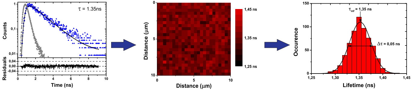
FIG. 1: (a) Typical decay curve measured for the FRET pair at 60 nm from a silver mirror (blue triangles), measured at 525 \pm 15 \text{ nm} . The solid black line is the single-exponential fit to the data. The grey circles correspond to the instrument response function (IRF) of the system. The residuals are plotted at the bottom and show the good quality of the fit in the whole decay range. (b) Typical lifetime image, showing a uniform distribution of the lifetimes. Each pixel represents the lifetime extracted from a fit similar to the one shown in (a). (c) The lifetime histogram obtained from the lifetime image in (b). The histogram shows a narrow Gaussian distribution indicating a good sample preparation.
