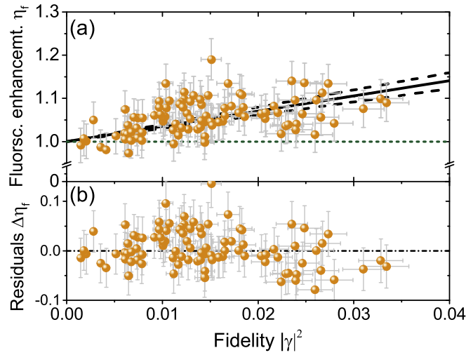
Figure 4. (a) Measured fluorescent power enhancement \eta_f versus the fidelity |\gamma|^2 for an L = 22.8 \mu\text{m} \pm 0.95 thick ZnO sample. The symbols are 100 experimental data points obtained at different positions on the sample. The vertical and horizontal error bars are 4% and 7% respectively (appendix A contains error estimation). The solid line is a linear regression through the data and the dashed curves delimit the 95% confidence interval. The green dotted line: \eta_f = 1 (b) residuals of the experimental data, that are randomly distributed about the linear model.
