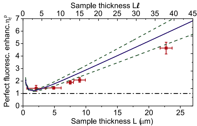
Figure 5. Fluorescent power enhancement \eta_f^p in ZnO scattering samples versus sample thickness. The red squares are the measurement-derived fluorescent power enhancement at perfect intensity control. The blue solid line is the calculated fluorescent power enhancement \eta_f^p from (4). The uncertainty in the fluorescent power enhancement \delta\eta_f^p is plotted as the two green dashed curves, which were calculated using equation (5). The black dashed-dotted curve is for an invariant distribution of energy density along the sample depth. Parameters to obtain the theoretical curves are given in table 1.
