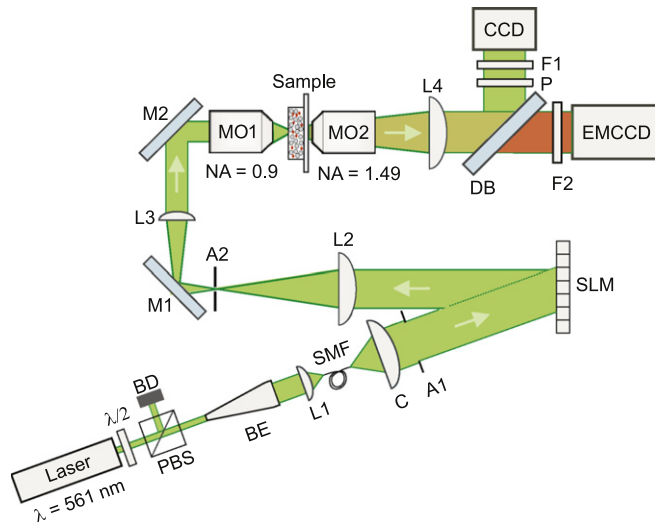
Figure 3. Experimental setup: a spatially filtered and expanded CW laser at 561 nm illuminates a spatial light modulator (SLM). The beam size on the SLM is 8 mm. A demagnified image of the surface of the SLM is focused onto a scattering sample of ZnO nanoparticles doped with fluorescent spheres. The back surface of the sample is imaged onto the EMCCD camera, which detects the fluorescent intensity and a CCD camera, which detects the excitation green laser light. The dichroic beam splitter separates the fluorescent intensity from the excitation beam. \lambda/2 is a half-wave plate, PBS is a polarizing beam splitter, BD is a beam dump, BE is a beam expander, L1, L2, L3, and L4 are lenses with focal distances of 11 mm, 200 mm, 100 mm, and 500 mm respectively, SMF is a single mode fiber, C is a collimator, A1 and A2 are apertures, M1 and M2 are mirrors, MO1 and MO2 are microscope objectives, DB is a dichroic beam splitter, F1 and F2 are filters, and P is a polarizer.
