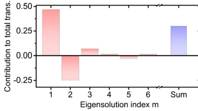
Figure 6. The contribution to the total transmission of the first six eigensolutions are represented by the red bars. The total transmission, that is the sum of the transmissions of all individual eigensolutions, is shown as the blue bar. Parameters: L = 8.33\ell , z_{e1} = 1.96\ell , z_{e2} = 0.68\ell .
