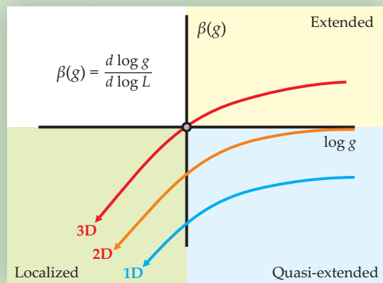
Figure 4. According to scaling theory, Anderson localization is a critical phenomenon, at least in three dimensions. The scaling function \beta(g) describes how—or more precisely, with what exponent—the average conductance g grows with system size L . For a normal ohmic conductor in D dimensions, the conductance varies as L^{D-2} ; consequently, \beta(g) \sim D - 2 for large g . Thus the beta function is positive for three-dimensional conductors, zero for two-dimensional conductors, and negative in one dimension. In the localized regime, g decays exponentially with sample size so that \beta(g) is negative. In three dimensions, that leads to a critical point at which \beta vanishes for some special value for g associated with the mobility edge. Lower-dimension systems do not undergo a genuine phase transition because the conductance always decreases with system size. A small 2D conductor, for instance, will look like a metal in the quasi-extended regime, but all its states are eventually localized if the medium is large enough.
