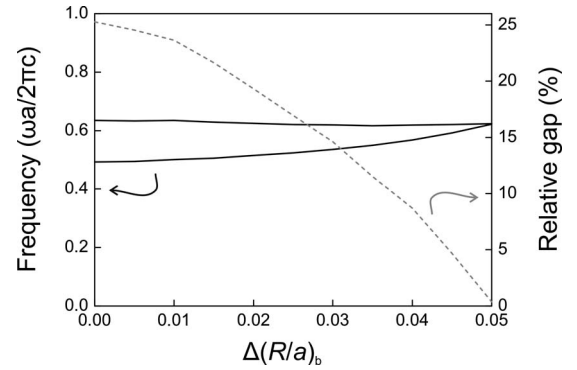
FIG. 6. Calculated relative width of the band gap (dashed line) and band gap edges (solid lines) for crystals with both (R_1/a) and (R_2/a) varying by opposite values from (R/a)=0.24 . Ratio (R_1/a) is increased, whereas (R_2/a) is decreased. Data is shown for \Delta(R/a)_b up to 0.05, calculated in 0.005 increments. The relative width of the band gap decreases as \Delta(R/a)_b increases. At a difference of \Delta(R/a)_b = 0.035 , the relative width of the band gap is halved. At a difference of \Delta(R/a)_b = 0.05 the band gap vanished. The center of the two band gap edges slightly increases as \Delta(R/a)_b increases.
