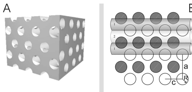
FIG. 1. (a) Three-dimensional representation of a cubic inverse woodpile photonic crystal. The alignment of the pores between the pores of the other set can be clearly seen, as well as the overlap of the pores. (b) Face-on view of the pores in the inverse woodpile photonic crystal. The centers of the perpendicular cylinders are aligned exactly between rows of cylinders of the other set. The individual pore sets have a centered rectangular lattice symmetry, with lattice parameters (a/c)=\sqrt{2} . An optimal photonic crystal is achieved when the ratio of radius R to lattice parameter a equals 0.24.
