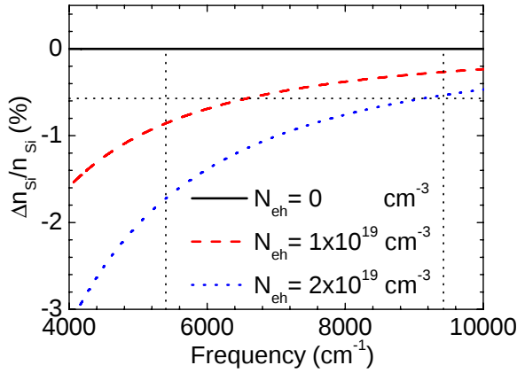
Figure 6.12: Relative refractive index change in Si versus probe frequency at three different carrier densities. The vertical dotted lines indicate the stop band edges \omega = 5400 \text{ cm}^{-1} and \omega = 9425 \text{ cm}^{-1} . The horizontal dotted line indicates the value \Delta n_{\text{Si}}/n_{\text{Si}} = 0.57\% that was obtained from Fig. 6.10.
