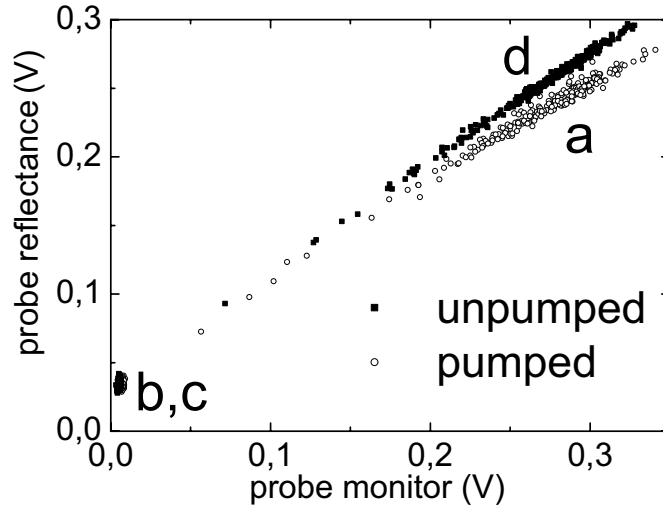
Figure 4.5: Reflectance signal versus monitor data for 1000 pulse events of the data set shown in Fig. 4.4 displayed as a scatter plot. The 250 unpumped reflectivity datapoints (d) constitute a line, indicating that that variations in monitor and reflectance signal are strongly correlated. The slope of the line is proportional to the reflectivity of the sample. The pumped datapoints (a) form a line with a reduced slope, due to the reflectivity decrease of about \delta R/R = 10\% in the switched sample. Both background data sets (b) and (c) tend to the origin of the plot as it should in absence of offsets. Note that the small offset in the signals is automatically removed in the data processing routine.
