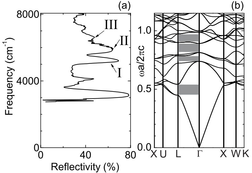
Figure 7.4: (a) Linear FT-IR reflectivity measurements with a NA= 0.28 Cassegrain objective, measured on position A (focal width \approx 75 \mu\text{m} ). The observed peaks in the range of second order Bragg diffraction are labeled I, II, and III. (b) Photonic dispersion relation organized into a band structure for fcc close packed air spheres (radius r=a/\sqrt{8} ) surrounded by spherical Si shells (radius 1.15r ) connected by cylindrical windows (radius 0.264r ). The volume fraction of solid material is about \Phi_{\text{Si}}= 21.3\% ( \epsilon_{\text{Si}}= 12.74 ). The frequency scale on panel (b) corresponds to the one on (a) for lattice parameter a= 1427 \text{ nm}
