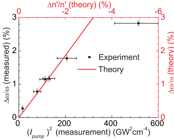
Figure 7.9: (symbols) Measured shift of the red edge of stop band I versus pump irradiance squared measured at a fixed reflectivity of R = 15\% at 1 ps after excitation. The pump frequency was \omega = 6450 \text{ cm}^{-2} . The quadratic scaling with irradiance confirms a two-photon excitation process. (curve) Calculated shift of the upper edge of the fifth band in the \Gamma -L direction in the band structure in Fig. 7.4 plotted versus \Delta n'_{Si}/n'_{Si} . The upper x axis was scaled such that the theory coincides with the measured data, directly relating the pump irradiance to the refractive index change.
