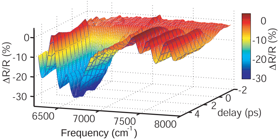
Figure 5.2: Differential reflectivity as a function of both probe frequency and probe delay \tau for the \lambda_c=1400 nm sample. The pump peak irradiance was I_0=310\pm1 GWcm ^{-2} . \tau was varied in steps of \Delta\tau=500 fs. The probe wavelength was tuned from 1255 to 1600 nm in \Delta\lambda=5 nm steps. Reflectivity increases of up to \Delta R/R=3.7\% at the blue edge of the stop band, as well as strong decreases of up to \Delta R/R=-30\% on the red edge of the stop band are observed. At 2 ps after excitation, the induced effect is stable.
