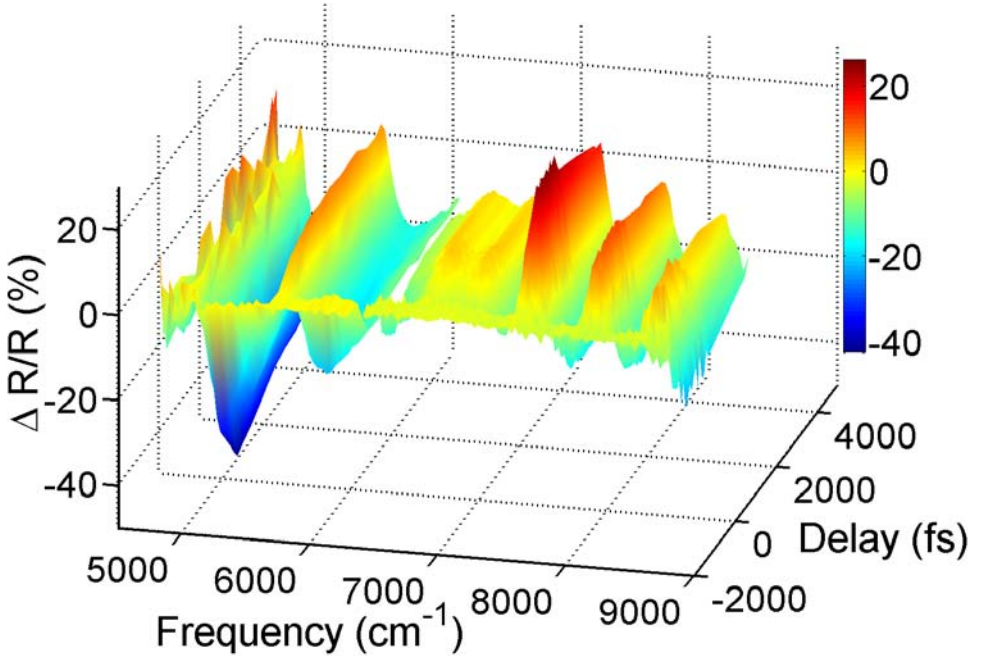
Figure 7.5: Differential reflectivity as a function of both probe frequency and probe delay. The pump frequency and peak irradiance were \omega_{\text{pump}} = 6450 \text{ cm}^{-1} and I_0 = 4 \pm 1 \text{ GWcm}^{-2} on the red part, and \omega_{\text{pump}} = 5000 \text{ cm}^{-1} and I_0 = 25 \pm 3 \text{ GWcm}^{-2} on the blue part of the spectrum. The probe delay was varied in small steps of \Delta t = 50 \text{ fs} on the blue edge and in steps of \Delta t = 500 \text{ fs} at the red edge. The probe wavelength was tuned from 1600 to 2100 nm in \Delta\lambda = 10 \text{ nm} steps in the low frequency range, and in 5 nm steps in the high-frequency range.
