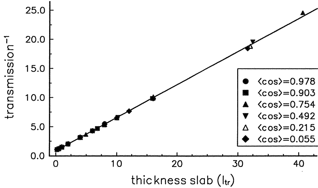
Figure 10: The inverse of the total transmission as a function of the thickness of the slab for various phase functions of the scatterers. The solid line is a numerical fit of Eq. (6.3).
