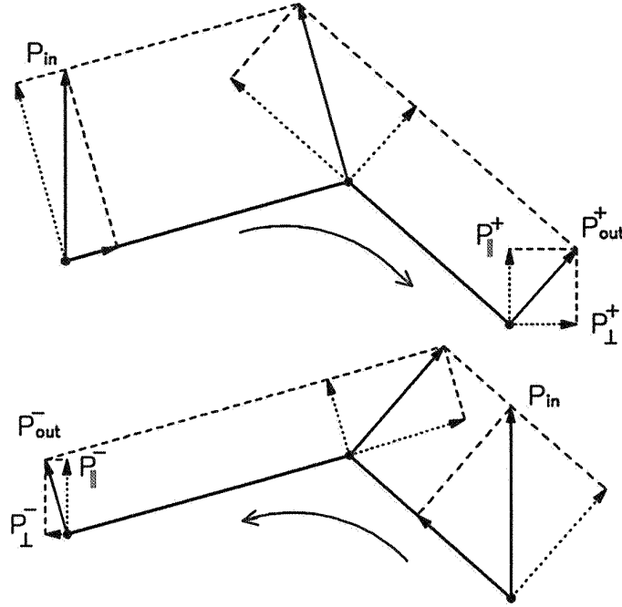
Figure 1: A triple scattering event for both propagation directions (time forward and time reversed), revealing additional phase shifts of the multiply scattered light. All scatterers and vectors lie in the plane of drawing. Each solid arrow denotes the amplitude of the electric field at that point, the dotted arrows are decompositions. It follows that P_{\parallel}^+ = P_{\parallel}^- , and P_{\perp}^+ \neq P_{\perp}^- .
