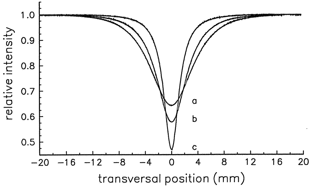
Figure 6: Transmitted intensity for various normal positions of an absorbent rod ( s=0.175 mm): a) z_0 = 5.90 mm, b) z_0 = 7.40 mm, c) z_0 = 9.00 mm. The experimental data are shown together with the best numerical fits for Eq. (7.32): a) z_0 = 5.67 \pm 0.05 mm, D_1/\alpha s = 1.11 \pm 0.03 ; b) z_0 = 7.14 \pm 0.05 mm, D_1/\alpha s = 1.04 \pm 0.03 ; c) z_0 = 8.39 \pm 0.05 mm, D_1/\alpha s = 0.95 \pm 0.03 . For all cases p = 0 , l_{tr} = 20 \pm 3 \mu m, L = 10.0 mm.
