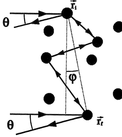
Figure 2: A scattering path contributing to the reflected intensity can be traversed in two directions as indicated by the arrows. The observation direction makes an angle \theta with the exact backscatter direction.
