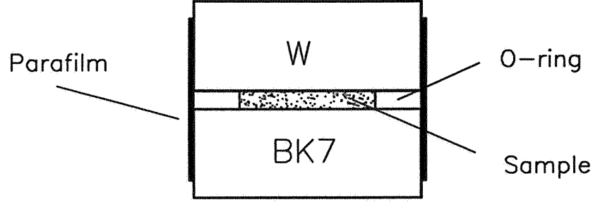
Figure 3: A suspension of TiO_2 -particles is sandwiched between two different windows. The backscatter cone can be recorded from either side. The windows are denoted by 'W', and 'BK7'.
