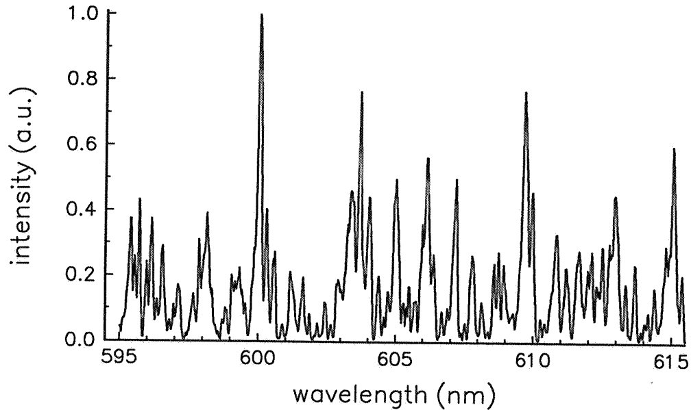
Figure 1: Transmitted intensity scattered in a small solid angle as a function of the wavelength of the light. Sample: TiO_2 -particles, average size: 270 nm, thickness sample: 14 \mu m .
