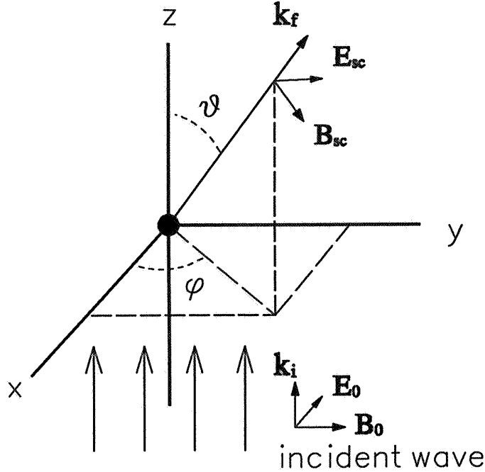
Figure 1: Incident light along the z-axis with wavevector \mathbf{k}_i is scattered in direction \mathbf{k}_f by a particle located at the origin, \mathbf{E} and \mathbf{B} denote the electric and magnetic field, respectively, of the incident and scattered light.
