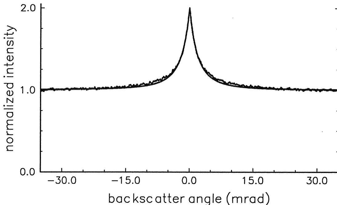
Figure 2: The backscattered intensity of an aqueous suspension of monodisperse polystyrene spheres, \phi = 0.265 \mu m . The thickness of the sample is 1.2 mm . Circularly polarized light has been used. The smooth curve is a calculation using diffusion theory yielding an enhancement factor of 2.005 \pm 0.005 .
