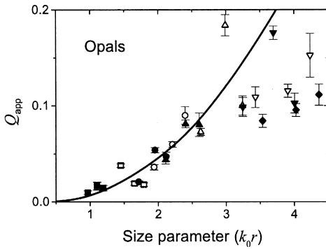
Fig. 4. The apparent scattering efficiency per sphere Q_{app} as a function of the size parameter, for radii 120 (■), 180 (□), 213 (●), 241 (○), 262 (▲), 326 (△), 403 (▼), 426 (▽), 439 nm (◆). The solid line is the Rayleigh–Gans scattering efficiency of a thin shell of refractive index 1 in an effective medium of refractive index 1.45 (see Footnote 4).
