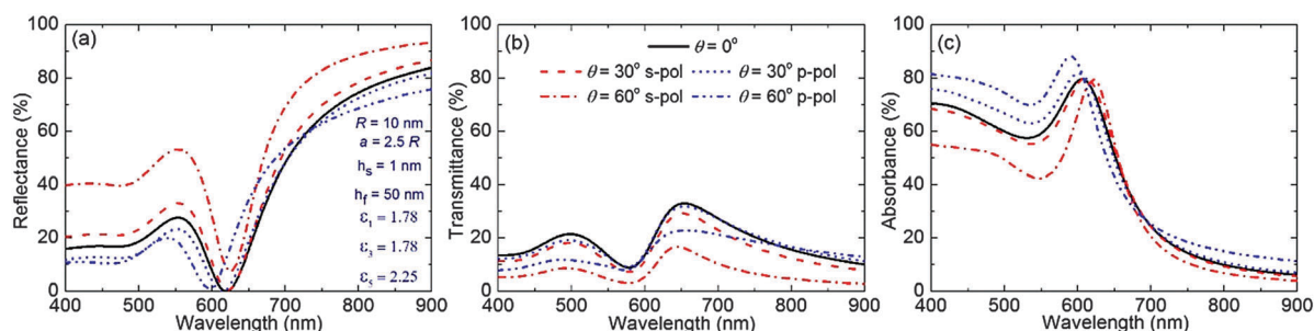
Fig. 6 Effects of incident angle and polarization of light on optical response spectra. Theoretically calculated optical spectra depicting reflectance (a), transmittance (b), and absorbance (c) at different incident angles \theta for s- and p-polarized light. All other system parameters are mentioned in (a).
