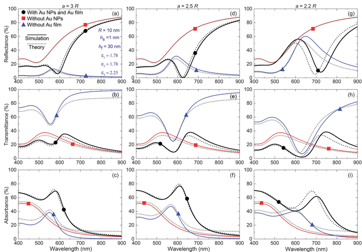
Fig. 2 Effect of the lattice constant on optical response spectra. Reflectance [top row], transmittance [middle row], and absorbance [bottom row] spectra (shown in black, denoted by circles) of a mirror-on-mirror structure calculated based on theory [dotted curves] as well as using numerical simulations [solid curves] as functions of lattice constant: a = 3R [left column], a = 2.5R [middle column], and a = 2.2R [right column]. Additional 'reference' spectra are included in each subplot: those obtained in the absence of gold (Au) nanoparticles (NPs) (shown in red, denoted by squares) and in the presence of NPs but the absence of the Au film (shown in blue, denoted by triangles). All other system parameters are mentioned in (a).
