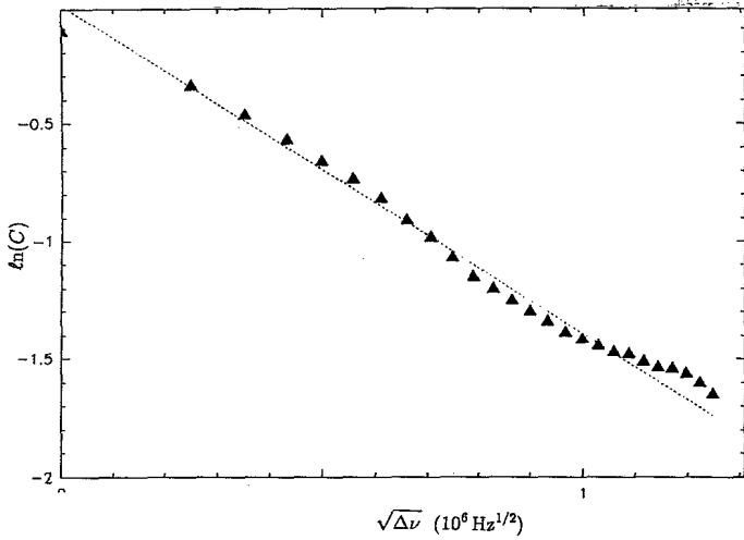
FIG. 2. Frequency-dependent intensity-intensity correlation in light backscattered from a sample of 36 vol% \text{TiO}_2 in air. Experimental points are averages over sixteen scans, probing different areas of the same sample. (Except for a slight flattening at small \Delta\nu that is due to the nonzero spectral linewidth of the source, no systematics is found in the "structure" of curves, obtained by probing different samples. This structure is therefore due to insufficient statistics.) The slope of the plot yields a value for the mean free time \tau . Determinations on a series of samples of different thicknesses yield an average value of \tau = 12.3 \pm 2.1 fs.
