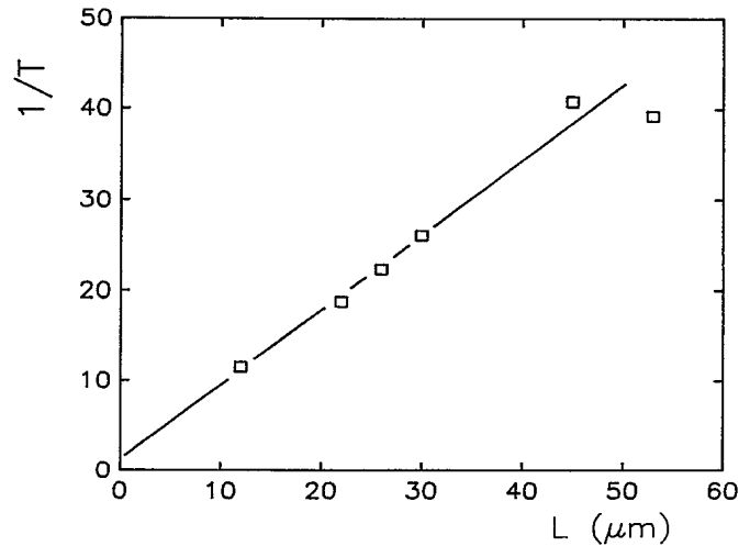
FIG. 1. Reciprocal of the total transmission through slabs of 36 vol% \text{TiO}_2 in air, as a function of slab thickness L . The straight line is a fit with diffusion theory and yields l=0.57 \pm 0.05 \mu\text{m} .
