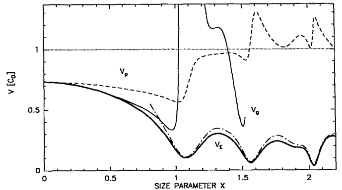
FIG. 4. Transport velocity for 36 vol% \text{TiO}_2 spheres in air ( n=2.73 ) as a function of the size parameter 2\pi a/\lambda , calculated from our microscopic theory (bold solid line) and inferred from energy-density arguments (dash-dotted line). Dashed line: phase velocity. Solid line: part of the strongly anomalous group velocity.
