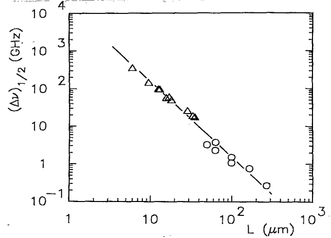
FIG. 3. Width at half maximum of the frequency-dependent intensity-intensity correlation in light transmitted through a sample of 36 vol% \text{TiO}_2 in air. From the figure we infer a diffusion coefficient D = 11.7 \pm 1 \text{ m}^2 \text{ s}^{-1} .
