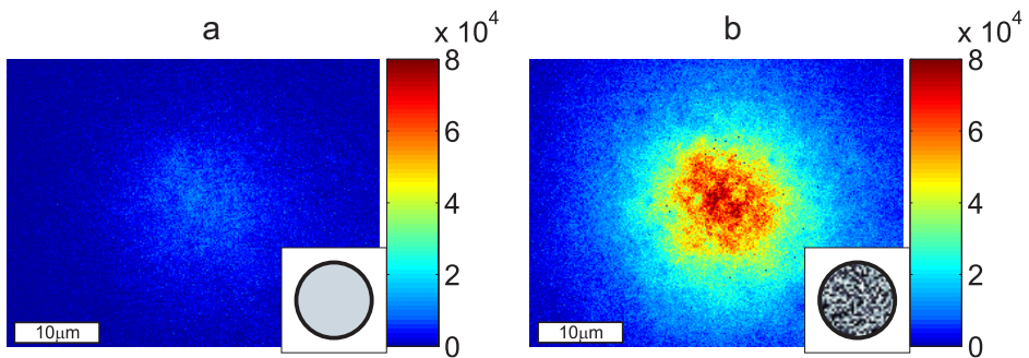
Figure 5.3: Experimental demonstration of channel demixing. a) Fluorescence image of a 300 nm sphere, embedded in ZnO pigment at a depth of 9.7 μm. Conventional illumination after a scan to find the position where the fluorescence is maximal; approximately 3 times the speckle average intensity. Inset, phase of the incident wavefront (plane wave). b) Our channel demixing method. Same sphere and sample position as in a) , the phases of the incident channels were set to the measured optimal values. The resulting fluorescence intensity has increased by a factor of 22 with respect to the average intensity. Inset, phase of the incident wavefront. Inside the sample this seemingly random wavefront transforms into a focus. Intensities are in counts per second.
