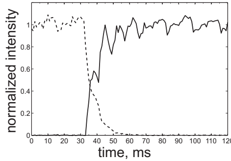
Figure 2.10: Transient intensity response of the LCD for switching the amplitude from 0 to maximum (solid curve) and for switching it back to 0 (dashed curve). During the first 33 ms (2 frames) the display does not respond at all. The intensity is normalized to the average intensity in the ‘on’ state.
