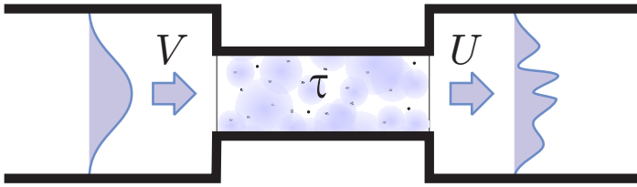
Figure 8.5: Diagrammatic representation of a sample in a medium with a higher refractive index. The sample supports fewer channels than the connecting waveguides and can, be thought of in a sense being ‘narrower’. Not all incident channels can couple into the sample.
