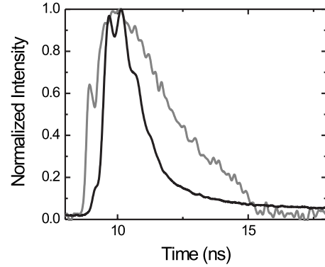
FIG. 1. Measured time traces of the pump pulse (gray) and emission output above threshold (black, input fluence = 0.47 \text{ mJ}/\text{mm}^2 ) of a titania random laser normalized to their maximum value. The pump pulse duration is much longer than the duration of the emitted light of the random laser above threshold. Relaxation oscillations in the emitted light are clearly visible near the peak intensity. The decay time of the emitted light is first dominated by stimulated emission. In the second part of the decay curve, spontaneous emission dominates.
