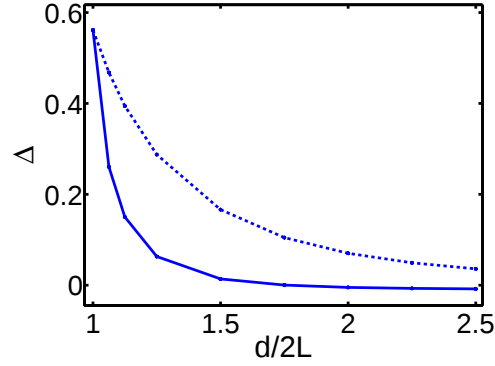
Fig. 5. The relative error \Delta versus normalized period of the cluster d/2L at wavelength \lambda = 14.5 \mu m . The solid line shows \Delta while the dashed one shows cubically decreasing function \sim (d/2L)^{-3} for comparison. The LDOS was calculated at the point x = 0.01 \mu m , y = z = 0 for the system consisting of 9 \times 9 \times 9 spheres with radius L = 0.01 \mu m and permittivity \epsilon_{sc} = 9 . The permittivity of the host medium is \epsilon_0 = 1 . The particles are arranged into simple cubic lattice centered at the point \mathbf{r} = 0 .
