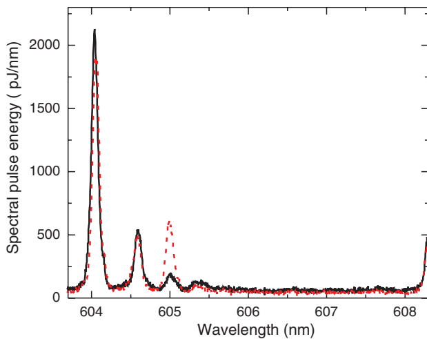
FIG. 1 (color). Two emission spectra of the random laser collected at the same spot on the sample. One spectrum (black) before and one (red) after shifting the sample by 37 \mu\text{m} and back. Apparently, the frequencies of the modes are fully determined by the realization of the disorder.
