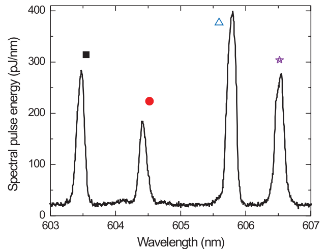
FIG. 2 (color). One of the 50 single-shot-emission spectra of our random laser system collected at one position of the sample. The symbols near the peaks correspond to the pulse energy of those peaks in Fig. 3.
