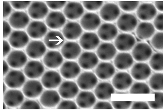
FIG. 1. High resolution SEM image of the Si inverse opal after HF etching. The scale bar is 2 \mu\text{m} . The arrow indicates an almost filled interstice in the structure. From this image we estimate the radius of the windows that interconnect the air spheres to be r_{\text{cyl}} = 0.16 \pm 0.05 r_{\text{sphere}} .
