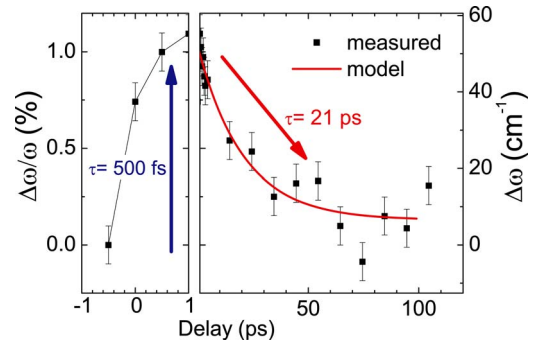
FIG. 3. (Color online) Blueshift of the low frequency edge of stop band I plotted versus probe delay (symbols). The pump frequency and irradiance were \omega = 6450 \text{ cm}^{-1} and 4 \pm 1 \text{ GW cm}^{-2} , respectively. The large shift amounts to \Delta\omega/\omega = 1.1\% with an exponential growth time of \tau = 500 \text{ fs} (left-hand panel). The subsequent exponential decay is well fitted with a single exponential decay \Delta\omega/\omega = A + \exp(-t/\tau) (red curve), where the decay time \tau = 21 \pm 4 \text{ ps} , and the small offset of \Delta\omega/\omega is A = 0.13\% (right-hand panel).
