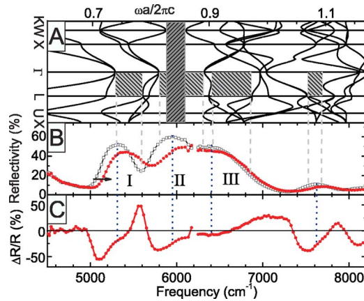
FIG. 2. (Color online) (a) Photonic band structures for fcc close packed air spheres (radius r = a/\sqrt{8} ) surrounded by spherical Si shells (radius 1.15) connected by cylindrical windows (radius 0.264r ). The volume fraction of solid material is about \Phi_{\text{Si}} = 21.3\% ( \epsilon_{\text{Si}} = 12.74 ). The frequency scale corresponds to the one in (b) and (c) for lattice parameter a = 1427 nm. The four light gray areas indicate stop gaps that occur in the \Gamma -L direction. The dark gray bar indicates the frequency range of the band gap. (b) Unswitched (open squares) and switched (closed circles) reflectivity spectra of the sample at normal incidence measured with our OPAs. The observed peaks in the frequency range of second order Bragg diffraction are labeled I, II, and III. In experiments on the red part of the spectrum ( \omega_{\text{probe}} < 6250 \text{cm}^{-1} ), the pump frequency was chosen to be \omega_{\text{pump}} = 6450 \text{cm}^{-1} . In experiments on the blue edge ( 6250 \text{cm}^{-1} < \omega_{\text{probe}} ), the pump frequency was reduced to \omega_{\text{pump}} = 5000 \text{cm}^{-1} . The pump irradiance for the switched spectrum was I_0 = 11 \pm 2 GW \text{cm}^{-2} on the red part and I_0 = 24 \pm 2 GW \text{cm}^{-2} on the blue part of the stop band. The switched spectra were measured at a pump-probe time delay of \approx 1 ps. We observe a large blueshift of up to 1.5% of the complete stop band in the range of second order Bragg diffraction as well as of features outside the stop band. (c) Differential reflectivity spectrum. A blueshift of peak I at \omega = 5320 \text{cm}^{-1} is illustrated by strong decreases and increases of the reflectivity below and above this frequency respectively. Similar dispersive curves are centered at frequencies of 5960 (II), 6450 (III), and 7600 \text{cm}^{-1} (vertical dotted lines).
