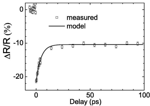
FIG. 4. (Color online) Differential reflectivity at \omega=5882 \text{ cm}^{-1} versus probe delay. The pump frequency and irradiance were \omega=6450 \text{ cm}^{-2} and 11 \pm 2 \text{ GW cm}^{-2} respectively. The large decrease amounts to \Delta R/R = -21\% within the first 500 fs, followed by a decay that is well fitted with a single exponential \Delta\omega/\omega = A + B \exp(-t/\tau) (curve), with amplitude B = -11\% , decay time \tau = 4.5 \pm 0.5 \text{ ps} and offset A = -10\% . The offset appears to decay slowly at ns times and is attributed to the wafer substrate.
