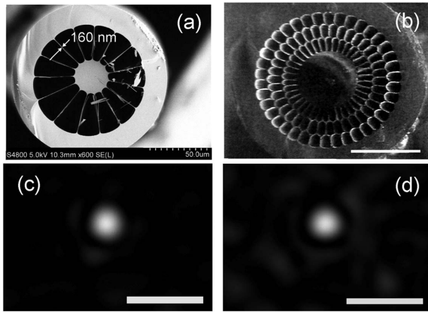
Fig. 3. Profiles of the PCF with a round core shape with a diameter \varnothing 28 \mu\text{m} and width of the suspending webs w = 160 nm (a) and with a diameter \varnothing 45 \mu\text{m} and width of the suspending webs w = 290 nm (b), and corresponding fiber outputs after wavefront shaping with \text{NA} \approx 0.59 (c) and \text{NA} \approx 0.61 (d). Scale bars are 50 \mu\text{m} (a), (b) and 2 \mu\text{m} (c), (d).
