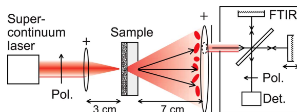
Fig. 1. (Color online) Experimental setup.
