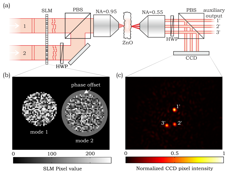
Fig. 3. Setup for wavefront-shaped optical circuits. (a) Two input modes (1, 2) are phase-modulated with a spatial light modulator (SLM). Both modes are spatially overlapped with a polarizing beam-splitter cube (PBS). The modes are focused on a layer of white paint (ZnO particles) that has been spray coated on a 1.5 mm thick microscope slide. The transmitted light is projected on a CCD camera. Three output modes 1', 2', and 3' are selected. (b) Optimized phase pattern on the SLM. A phase offset is applied to the second incident mode. (c) Camera image for three optimized spots when both input modes are incident on the phase pattern of (b).
