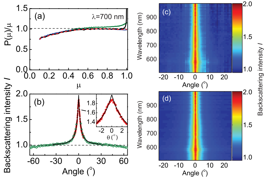
Fig. 2. (color online) (a) Diffuse angular transmission function P(\mu)/\mu against \mu = \cos(\theta) in backscattering, at \lambda = 700 nm, for (black line) TiO 2 and (blue line) tefflon, both helicity conserving channel, (green line) TiO 2 helicity nonconserving channel, and (dashed red line) TiO 2 linear-polarization nonconserving channel (averaged over s and p output polarizations). (b) EBS of TiO 2 sample at \lambda = 700 nm, normalized to linear-polarization nonconserving channel of TiO 2 , measured using configuration (i) (open diamonds, green) and configuration (ii) (squares, red), and fit using Eq. (2) (black line). Inset: detail of (b) around cone center. (c) Color density plot showing enhanced backscattering intensity from the TiO 2 powder sample over a wavelength range of 520-1000 nm. (d) Same for fitted EBS cones using Eq. (2).
