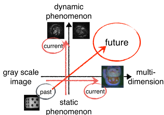
Figure 3. Progress in digital holography; from a gray scale image to a multi-dimensional image, and from a static phenomenon to a dynamic phenomenon.
