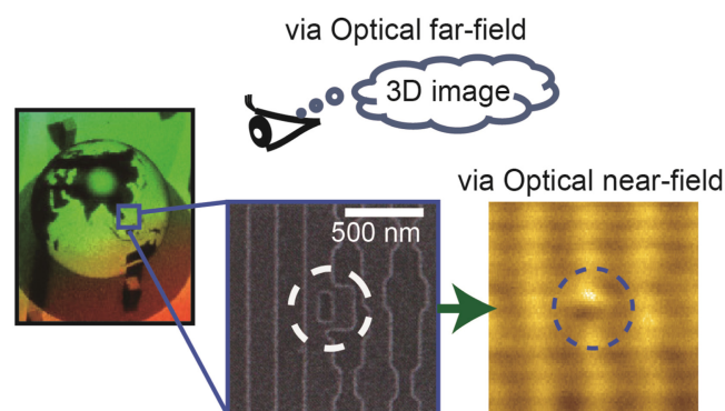
Figure 16. Hierarchical hologram that acts as a conventional hologram in the optical far-field but contains additional information retrieved only via optical near-fields.
