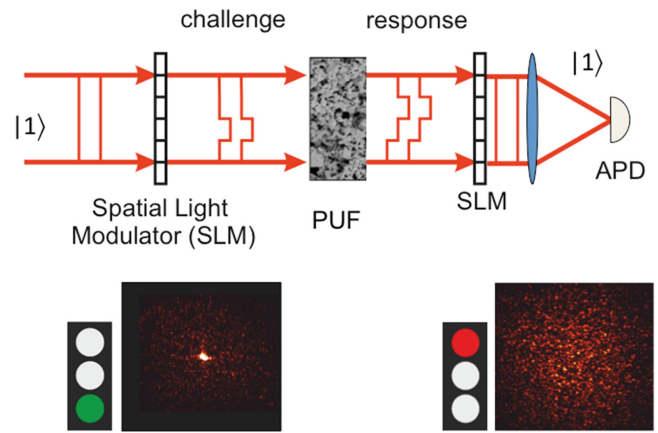
Figure 23. Schematic of quantum secure authentication [145]. A few-photon wavefront is shaped into a complex wavefront by an SLM. The response is transformed again with another SLM such that only with the correct key, the output light will be focussed to a point, where an APD behind a pinhole measures the amount of light falling into the target spot. With the wrong key, the output is a speckle pattern that will result in a much lower signal.
