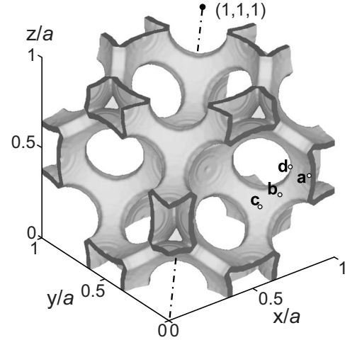
Fig. 5. Rendering of the dielectric function in one fcc unit cell that models the \text{TiO}_2 inverse-opal structure in Section 4: an fcc lattice of air spheres of radius r=0.25\sqrt{2}a with a being the cubic lattice parameter. The spheres are covered by shells with \epsilon=6.5 and outer radius 1.09r . Neighboring air spheres are connected by windows of radius 0.4r . The letters a–d indicate four different positions at the \text{TiO}_2 –air interface: a =(1,0,0)/(2 \sqrt{2} ), b =(1,1,2)/(4 \sqrt{3} ), c =(1,1,1)/(2 \sqrt{6} ), d =(0.33,0.13,0) (points shown are symmetry-equivalents). The dashed-dotted line shows the body diagonal of the cubic unit cell.
