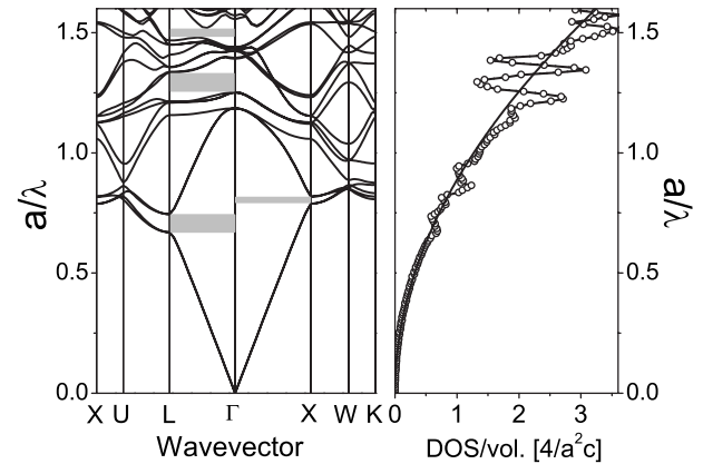
Fig. 6. Left side: Photonic band structure (Media 2) for the \text{TiO}_2 inverse opal shown in Fig. 5. The gray rectangles indicate stopgaps in the \Gamma L direction and one stopgap in the \Gamma X direction for the inverse opal. Right side: The stopgaps result in the decreased DOS as shown by open circles (Media 3) at corresponding frequencies compared to the DOS in a homogeneous medium with n_{av}=1.27 as shown by the solid curve.
