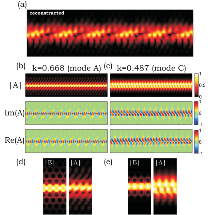
FIG. 3. (Color online) (a) Reconstructed amplitude for Fig. 2(a) using Bloch modes m=4 and m=5 only. (b and c) Amplitude, imaginary part, and real part for both Bloch modes. (d and e) Comparison between calculated |E| (left) and reconstructed |A| (right).
