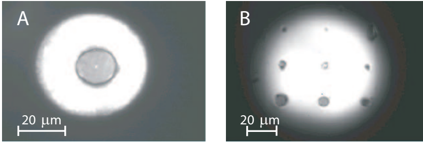
FIGURE 7.3: (A) Microscope image of a micropillar cavity with 20\ \mu\text{m} diameter. The image is made with a microscope consisting of a reflecting microscope objective with NA 0.65 and a 200 mm tube lens. White and black corresponds to a high and low light intensity, respectively. The white circular area is the illuminated part of the sample. The pillar appears as a grey circle with a dark edge. The dark edge corresponds to the gold coating. The white spot in the center of the pillar is focussed white light from the probe beam. (B) Microscope image of a field of pillars using a refracting microscope objective with NA 0.65 and a 100 mm tube lens. Pillars with a diameter between 4\ \mu\text{m} and 10\ \mu\text{m} and the base of pillars with a diameter of 1\ \mu\text{m} and 3\ \mu\text{m} are visible. The focussed probe beam impinges on the center pillar with diameter 4\ \mu\text{m} .
