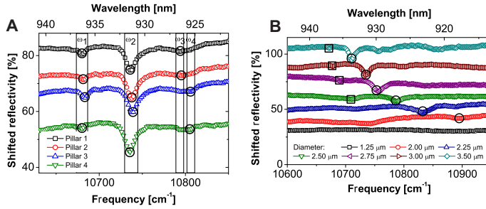
FIGURE 7.10: Reflectivity spectra of the cavity resonance for uncoated micropillar cavities with (A) 3 \mu\text{m} diameter. The reflectivity axis has been offset with steps of 10% except for the lowest. Each resonance is indicated with a bold circle. The center frequency of the resonances shows little variation among different pillars of the same diameter (within vertical lines). (B) Reflectivity spectra of the cavity resonance for micropillar cavities with diameters between 1.25 \mu\text{m} and 3.5 \mu\text{m} . The reflectivity axis has been offset. Resonances are indicated with bold squares and bold circles. A clear evolution of the resonances is visible: the frequency of a resonance increases with decreasing pillar diameter, as well as the resonance spacing. The reflectivity spectra for pillars with 2 \mu\text{m} diameter and smaller show weakly pronounced resonances or no resonances at all.
