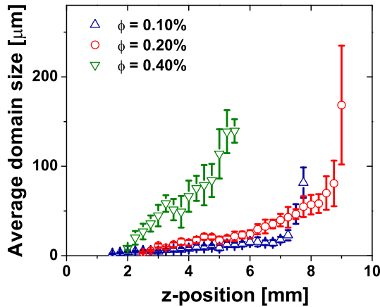
FIGURE 10.7: Average domain size of opals grown at different volume fractions at T = 309\text{ K} as a function of the z -position on the sample. An increase of average domain size towards the bottom of the substrate is observed for all three volume fractions.
