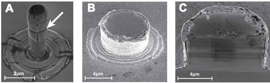
FIGURE 7.1: (A) SEM image of a micropillar cavity with 1\ \mu\text{m} diameter and a height of 5.7\ \mu\text{m} . At the pillar edge one can see an alternating light- and dark-gray color pattern associated to the GaAs/AlAs Bragg stack with 13\ \lambda/4 layer pairs, a GaAs \lambda cavity layer, and a second Bragg stack with 25\ \lambda/4 layer pairs. The \lambda cavity is indicated with a white arrow. (B) SEM image of a pillar with 8\ \mu\text{m} diameter. The substrate and the pillar edge are covered with gold. The top facet is clean. The alternating pattern on the edge is associated to the GaAs/AlAs Bragg stack with 12\ \lambda/4 layer pairs, a GaAs \lambda cavity layer, and a second Bragg stack with 16\ \lambda/4 layer pairs. At the base of the pillar a ring pattern is visible. (C) Cross section of a cleaved gold-coated pillar with 8\ \mu\text{m} diameter. The GaAs/AlAs Bragg stack with 12\ \lambda/4 layer pairs, a GaAs \lambda cavity layer, and a second Bragg stack with 16\ \lambda/4 layer pairs are clearly visible.
