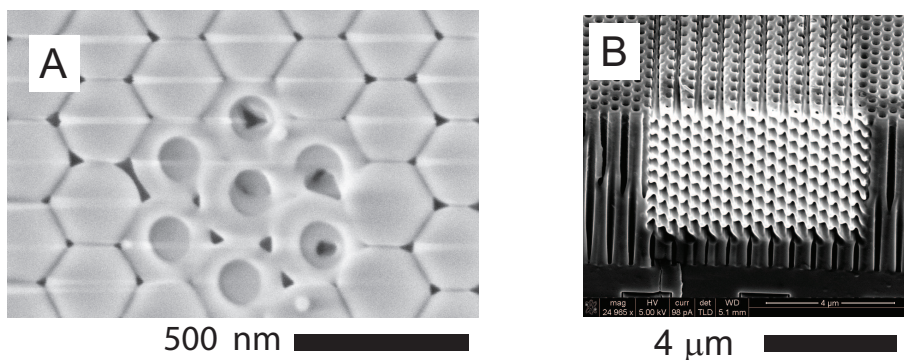
FIGURE 1.10: (A) Scanning electron micrograph of a silica opal with an intentional point defect that will act as a cavity [33]. The silica opal functions as a mirror. The mirror around the cavity becomes three dimensional if a second layer of opal photonic crystal is grown on top of the layer shown in the micrograph. (B) Scanning electron micrograph of a three-dimensional silicon photonic crystal. The larger array of vertical pores is etched using reactive ion etching, while the horizontal set of pores is etched using a focussed ion beam [34].
