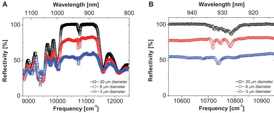
FIGURE 7.6: (A) Reflectivity spectra of three different micropillar cavities with 20 \mu\text{m} , 6 \mu\text{m} , and 3 \mu\text{m} diameter. The reflectivity of the stopband decreases with decreasing pillar diameter. For pillars with diameter 6 \mu\text{m} and smaller the stopband is not perfectly flat. (B) A zoom-in on the cavity resonances of figure (A). The plots show 7, 3, and 2 troughs (resonances) at the cavity resonance of pillars with 20 \mu\text{m} , 6 \mu\text{m} , and 3 \mu\text{m} , respectively. The total number of resonances decreases, but the resonance spacing increases with decreasing pillar. The cavity resonance of the 20 \mu\text{m} pillar is asymmetric: it is steeper at the blue side than at the red side.
