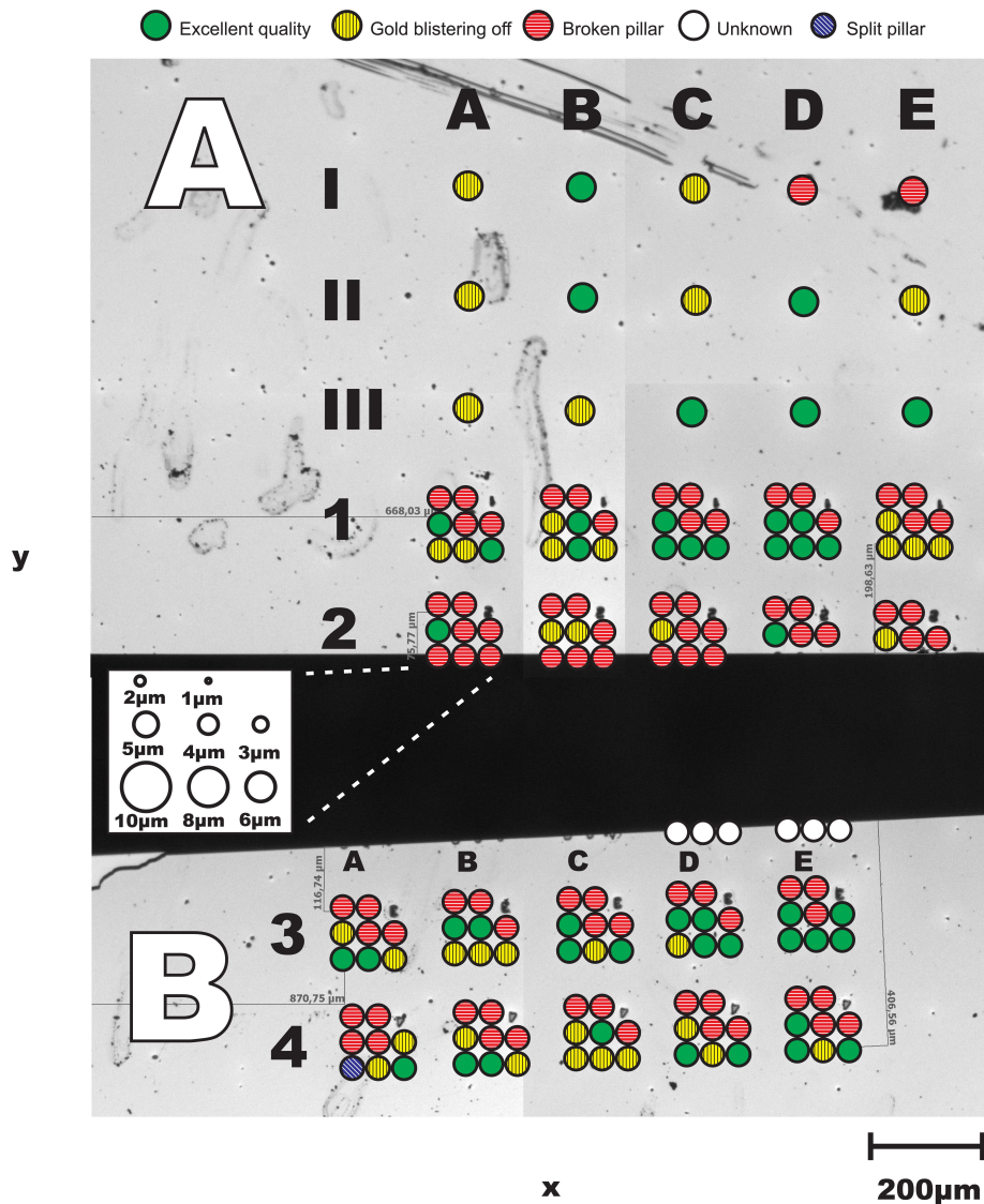
FIGURE 7.2: Map of a sample containing gold-coated micropillars. Four optical microscope images are merged to create the figure. The upper three rows contain pillars with diameter 20 \mu\text{m} . The fields having 8 circles contain pillars with diameters between 1 \mu\text{m} and 10 \mu\text{m} . A homogeneously filled green circle indicates the position of an "excellent" micropillar. A vertically patterned yellow circle is a "blistered" pillar and a horizontally patterned red circle is a "broken" pillar. The diagonally patterned blue circle indicates a pillar that is cut in half. The status of the pillars located at the six white circles is unknown.
