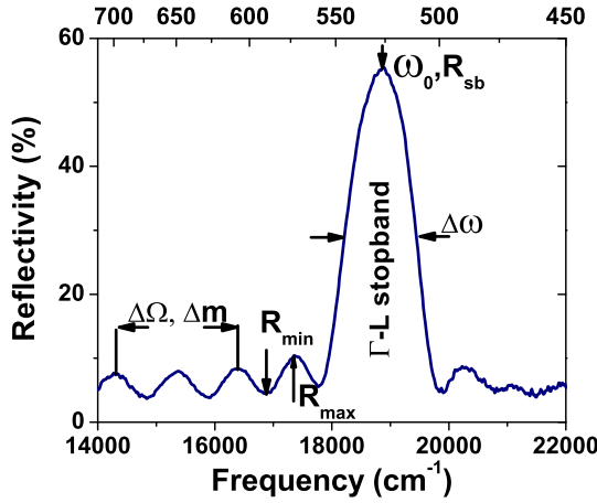
FIGURE 10.2: The reflectivity spectrum shows a first order stopband and Fabry-Pérot fringes. The high reflectivity peak of 55% at 18880 \text{cm}^{-1} is the result of the \Gamma - L stopband. The frequency difference between \Delta m Fabry-Pérot fringes is indicated by \Delta\Omega . Here \Delta m = 2 and \Delta\Omega = 2083 \text{ cm}^{-1} are indicated.
