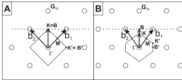
FIGURE 9.1: Representation of the first Brillouin zone for a square (A) and a \sqrt{2} -lattice (B), having a lower symmetry than the square lattice. The vectors b_1, b_2 are primitive vectors of the reciprocal spaces, while G_{11} is a reciprocal lattice point equivalent to the \Gamma point ( hk=11 ). \Gamma, K, K', B, B' and M are points of high symmetry of the Brillouin zone. The dotted lines are the hk=11 Bragg planes.
