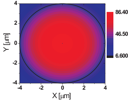
FIGURE 8.7: Calculated mode profile of fundamental micropillar mode HE11, 2R=8 \mu m . The colorscale indicates the absolute value of the electric field. The black circle indicates the pillar edge. The fundamental mode has a field maximum in the middle of the pillar. The field amplitude decreases towards the edge of the pillar.
