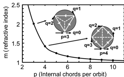
Fig. 2. Relative refractive index of the sphere for a geometrical resonance as a function of p for N = 1 .
