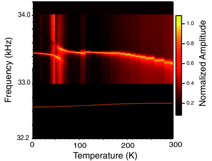
Figure 3. Measurement of the amplitude of the oscillation of a bare tuning fork (lower curve) and of a tuning fork with an attached fibre (upper curve) versus frequency and temperature. The change in the resonance frequency and width is significant in the second case.
