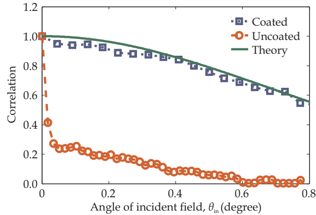
Figure 4. Influence of a Si anti internal-reflection coating on the correlation range of scattered light inside a GaP HIRES-lens when we change the angle \theta_{in} under which the beam incidents. The correlation range determines the Field of View of the lens and should therefore be as large as possible. In an uncoated GaP HIRES lens internal reflections significantly reduce the correlations. By coating the lens with a thin layer of amorphous Si these reflections are suppressed resulting in a much larger correlation range. The green solid line represents theoretical loss of correlation due to the optical memory effect.
