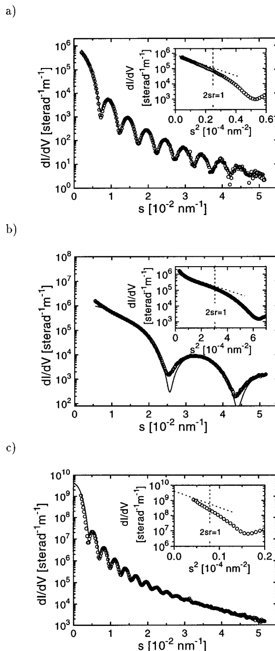
Figure 2. Differential scattering cross section dI/dV as a function of the scattering vector s = 2 \sin(\theta)/\lambda of dilute suspensions of spheres, plotted semilogarithmically (circles): (a) polystyrene in methanol (PS5020A); (b) microemulsion-grown silica in dimethylformamide ( \mu Ec1); (c) Stöber-grown silica in water (SC200). The presence of a large number of fringes indicates that the sizes of the spheres are highly monodisperse. The solid lines are model curves for spheres of homogeneous internal density. The inset shows the cross section as a function of s^2 , at low s (Guinier-plot). The dashed lines with a slope of (2\pi r)^2/5 have been drawn using the radii deduced from the fringe period.
