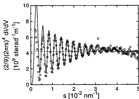
Figure 3. Differential scattering cross section dI/dV as a function of scattering vector s = 2 \sin(\theta)/\lambda (cf. Figure 2), plotted on a linear scale and multiplied by s^4 (Porod plot). (a) polystyrene in methanol (PS5020A); (b) microemulsion-grown silica in dimethylformamide ( \mu Ec1); (c) Stöber-grown silica in water (SC200). The polydispersity can be determined from the fringe amplitude (arrow) as a function of s . If the scattering cross section is multiplied by (2/9)(2\pi sr)^4 instead of s^4 , then the average height of the fringes (dotted line) yields the cross section in the forward direction ( s = 0 ), cf. inset in Figure 2. The solid lines are model curves for spheres of homogeneous internal density, taking into account size polydispersity and detector blurring.
