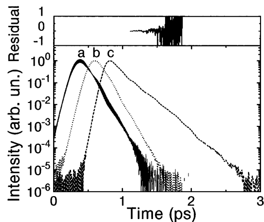
FIG. 1. Typical result of a time-resolved measurement of the transmitted pulse on a 1.43 \mu\text{m} sample [solid line, indicated with (a)]. The intensity of the pulse is plotted as function of time. The dotted line (b) shifted in time represents the Fourier filtered signal to which an exponential function was fitted: decay time \approx 70 fs. The relative residual between the determined and measured signal is shown on top of the figure. The dashed line (c) shows the result of a measurement on a 4.4 \mu\text{m} sample, demonstrating the exceptionally high dynamic range of 5 orders of magnitude.
