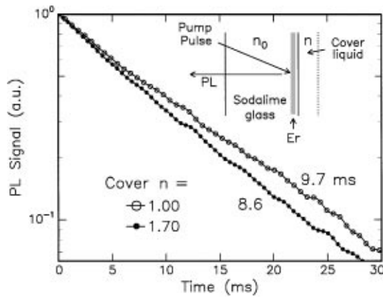
FIG. 2. PL decay traces of the 1.537 \mu\text{m} emission from sample A on a logarithmic scale. The solid data points were measured with a methylene-iodide film ( n = 1.70 ) covering the surface, the open data points in air. The inset shows how the luminescence signal was collected at the back of the sample, while the Er-doped front side was covered with various liquids with index n .
