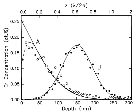
FIG. 1. Erbium concentration profiles as determined with RBS (open and solid data points). The drawn lines are deconvoluted for the detection resolution. The top axis shows the distance in units of \lambda/2\pi (where \lambda = 1.537\ \mu\text{m} is the spontaneous emission wavelength in vacuum).
