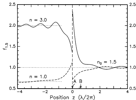
FIG. 4. Polarization- and angle-averaged local classical density of optical modes, on both sides of an interface between infinite half-widths. The refractive index on one side is n_0 = 1.50 . Calculations are shown for n = 1.00 and 3.00 on the other side. The arrows indicate the locations of the Er profiles.
