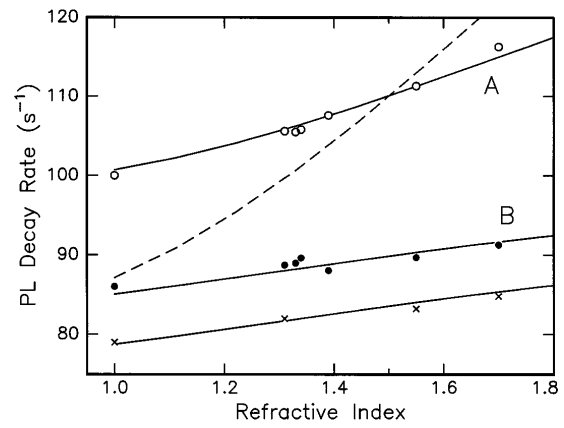
FIG. 3. Measured PL decay rates as a function of refractive index n of the cover liquids. The index of the sodalime glass is n_0 = 1.50 . Data are shown for both samples A (open data points) and B (solid data points). The \times symbols represent data from sample B measured one year later. The solid lines are calculations using Eq. (8); the dashed line shows a calculation assuming only radiative decay.
