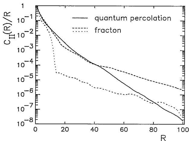
FIG. 3. Autocorrelation functions of probability distributions on 200 \times 200 percolating clusters. C_H is normalized at R=0 .
