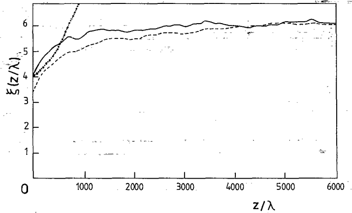
FIG. 2. A measure of the width of the wave field \xi(z) (in units of \lambda ) as a function of the length of the sample z . Solid line: Estimate based on the second moment of |\psi(x,y,z)|^2 . Dashed line: Estimate obtained from the knowledge of the fourth moment of |\psi(x,y,z)|^2 . Dots: \xi(z) for a uniform medium with the same estimator as for the solid line.
