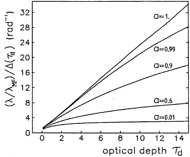
FIG. 13. The value (\lambda/\lambda_{MF})/\Delta(\tau_d) , associated with a difference slab of infinitesimal thickness at an optical depth \tau_d , is plotted against \tau_d for five different values of the albedo a . Notice that for a=1 the curve is a straight line which goes through the abscissa at \tau_d \approx -0.5 . Experimental results are given in Fig. 21.
