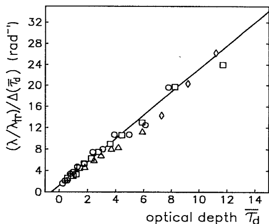
FIG. 21. (\lambda/\lambda_{tr})/\Delta(\bar{\tau}_d) vs \bar{\tau}_d for difference slabs in samples of different volume fractions of \text{TiO}_2 particles in 2-methylpentane-2, 4-diol. \circ , 0.36 vol %; \square , 1.05 vol %; \triangle , 2.50 vol %; \diamond , 9.81 vol %. Solid line: (\lambda/\lambda_{tr})/\Delta(\bar{\tau}_d) = 2.2(\bar{\tau}_d + 0.5) . See also Fig. 13.
