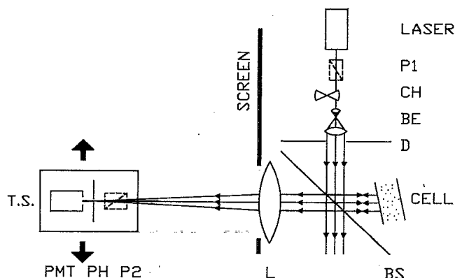
FIG. 18. Experimental setup for the observation of backscattering enhancement. P1 , P2 , polarizers; CH , chopper; BE , beam expander; BS , beam splitter; L , lens; PH , pinhole; TS , translation stage.
