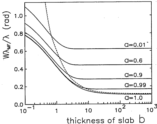
FIG. 12. The value W(\lambda_{MF}/\lambda) is plotted against the optical thickness b . The solid lines give the results from the diffusion approximation for five different values of the albedo. The dashed curve gives the result for the exact theory with a=1 .
