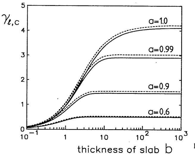
FIG. 9. Absolute values of \gamma_{l,c} at exactly backscattering [ \gamma_l(\mu_s = \mu_i, \mu_i) = \gamma_c(\mu_s = \mu_i, \mu_i) ] with \mu_i = 1 , as a function of the optical thickness b . Dashed curves represent the result from the exact theory as derived in Sec. II, solid lines give the result from the diffusion approximation. Different curves correspond to different albedos.
