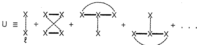
FIG. 5. Lowest-order contributions to the irreducible vertex U .
