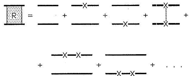
FIG. 4. Lowest-order contributions to the total vertex R .
