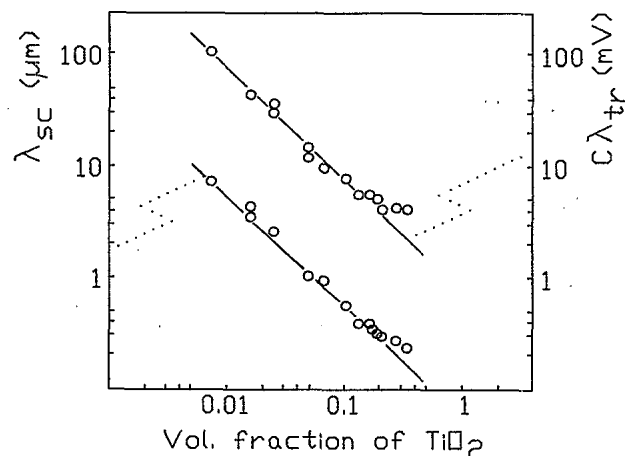
FIG. 17. Scattering mean free path (lower plot) and (upper plot) transport mean free path times a constant (see text) as a function of the volume fraction of \varnothing \approx 220 -nm \text{TiO}_2 particles.
