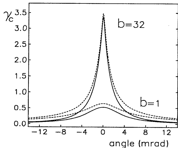
FIG. 10. Comparison of the absolute line shapes \gamma_c(\mu_s, \mu_i = 1) as found from the exact theory (dashed lines) and the diffusion approximation (solid lines) for slab thickness b = 32 and b = 1 , \lambda_{MF}/\lambda = 53.5 , and albedo a = 1 .
