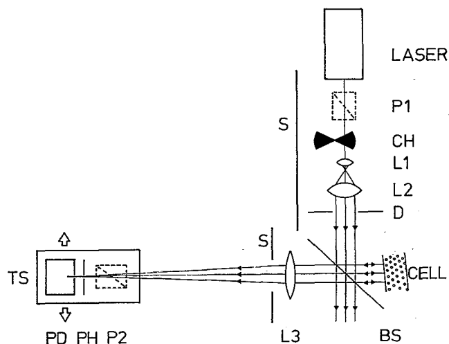
FIG. 1. Schematic representation of experimental setup. P1, P2, polarizers; CH, chopper; L1, L2, L3, lenses; D, diaphragm; BS, beam splitter; S, screen; TS, translation stage; PD, photodetector; and PH, pinhole.
