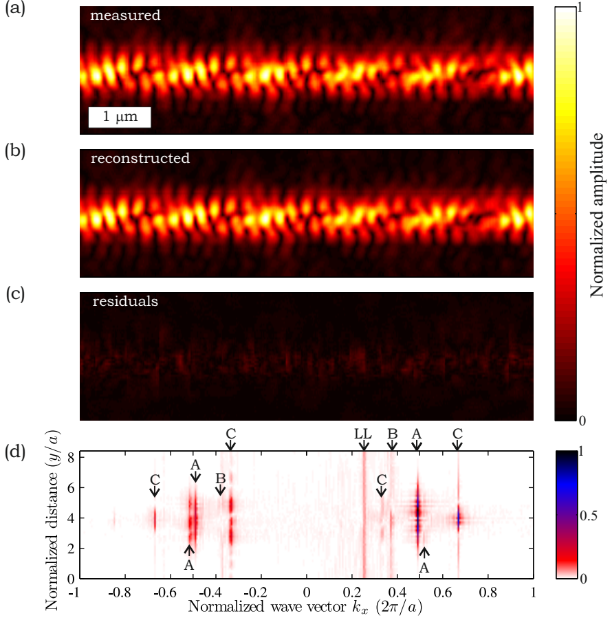
Figure 4.2. Reconstructed Bloch modes of a measured near-field pattern on a photonic-crystal waveguide. (a) Measured amplitude for a photonic-crystal waveguide at 931.6 \pm 0.1 \text{ nm} . (b) Fitted amplitude using 7 reconstructed Bloch modes over 30 unit cells. (c) Residual amplitude. (d) Amplitude coefficients of the spatial Fourier transforms of the measured near-field pattern. Labels correspond to those in Fig. 6.1(b).
