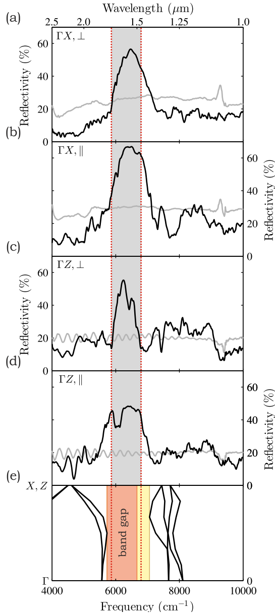
Figure 3.4. Measured reflectivity of an inverse woodpile photonic crystal. (a – d) Measured reflectivity (black lines) along two orthogonal directions (centered on \Gamma X and \Gamma Z ) and orthogonal polarizations (perpendicular \perp and parallel \parallel to the pores perpendicular to the measurement axes). The overlapping frequencies of the stop bands (gray bar) reveal the presence of a photonic band gap. Reference reflectivity (gray lines) are measured on non-photonic parts of the sample within 5 \mu\text{m} from the photonic crystal. (e) Calculated band structure for both \Gamma X and \Gamma Z reveal a stop gap (yellow bar), which is part of the band gap (orange).
