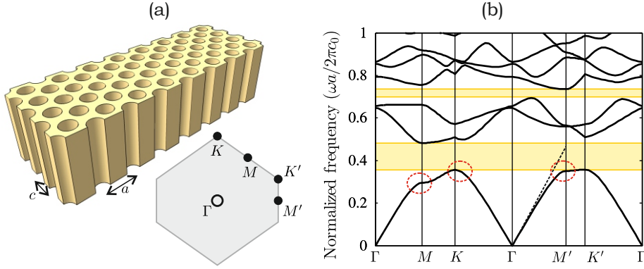
Figure 1.1. Geometry and dispersion of a two-dimensional photonic crystal. (a) Geometry of a macroporous two-dimensional silicon photonic crystal with a centered-rectangular lattice with a unit cell with long side a , short side c and pore radius r . The bottom shows the corresponding Brillouin zone in reciprocal space, where the labels mark points of high symmetry. (b) Calculated band structure for r/a = 0.225 and a/c = 1.41 for transverse-electric (TE) polarized light. The band structure shows two two-dimensional band gaps for TE-polarized light (yellow bars) and regimes that sustain slow-light propagation (red encircled areas). The dashed diagonal line indicates a fraction of the dispersion for rectilinear plane wave propagation in a homogeneous medium with constant effective refractive index similar to the one of the crystal.
