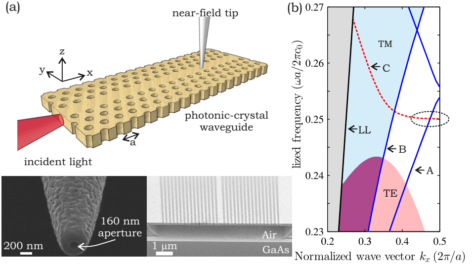
Figure 5.1. Experimental scheme for studying light transport in photonic-crystal waveguides. (a) Laser light is side-coupled on a GaAs photonic-crystal waveguide. Light propagation is studied with a near-field tip. SEM images are shown of the coated near-field tip (left) and the waveguide (right). (b) Calculated band structure showing both TE-like (red dashed) and TM-like (blue) guided modes in the 2D band gap for TE-like modes for (r/a = 0.303, h/a = 0.67) . The encircled area is the main focus of this chapter. Here, the TE-like waveguide mode C becomes flat at the band edge, leading to a Van Hove divergence in the DOS. The black diagonal line represents the light line ( LL ).
