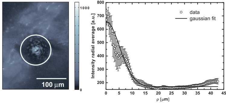
Figure 4.4: (left) Image of the 100\ \mu\text{m} pinhole taken in order to check the alignment of the setup. The bright spot in the center is the image of the focused He-Ne spot collected at the back of the sample. This image shows that the pinhole does not distort the speckle pattern produced by the sample. (right) The radial average of the central part of the image on the left is shown. The diameter of the focused spot on the back of the sample can be estimated to be on the order of 14\ \mu\text{m} . In order to collect the image we illuminate the pinhole with white light, as it is clear from the illuminated spot and that gives an intensity background higher than zero.
