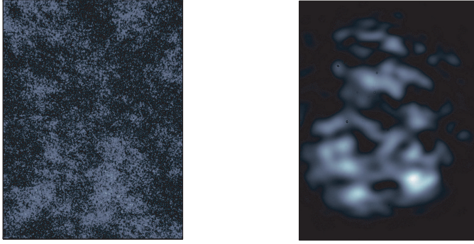
Figure 4.3: (left) Speckle pattern observed when there is no filtering pinhole. (right) Speckle pattern generated when the 100\ \mu\text{m} pinhole is in place. The pinhole prevents the formation of an additional speckle pattern, due to the sample substrate, superimposed onto the speckle pattern produced by the sample.
