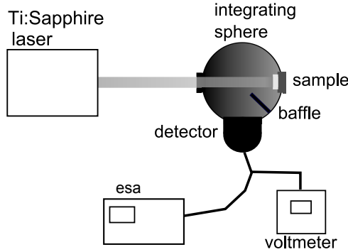
Figure 2.3: Sketch of the experimental setup used to measure total reflection of both classical and quantum noise. A Ti:Sapphire laser and an integrating sphere are used as source and to collect the reflected light, respectively. The baffle is needed to prevent specularly reflected light from hitting the detector. An electronic spectrum analyzer is employed to measure the noise content of the signal and a voltmeter to measure its intensity.
