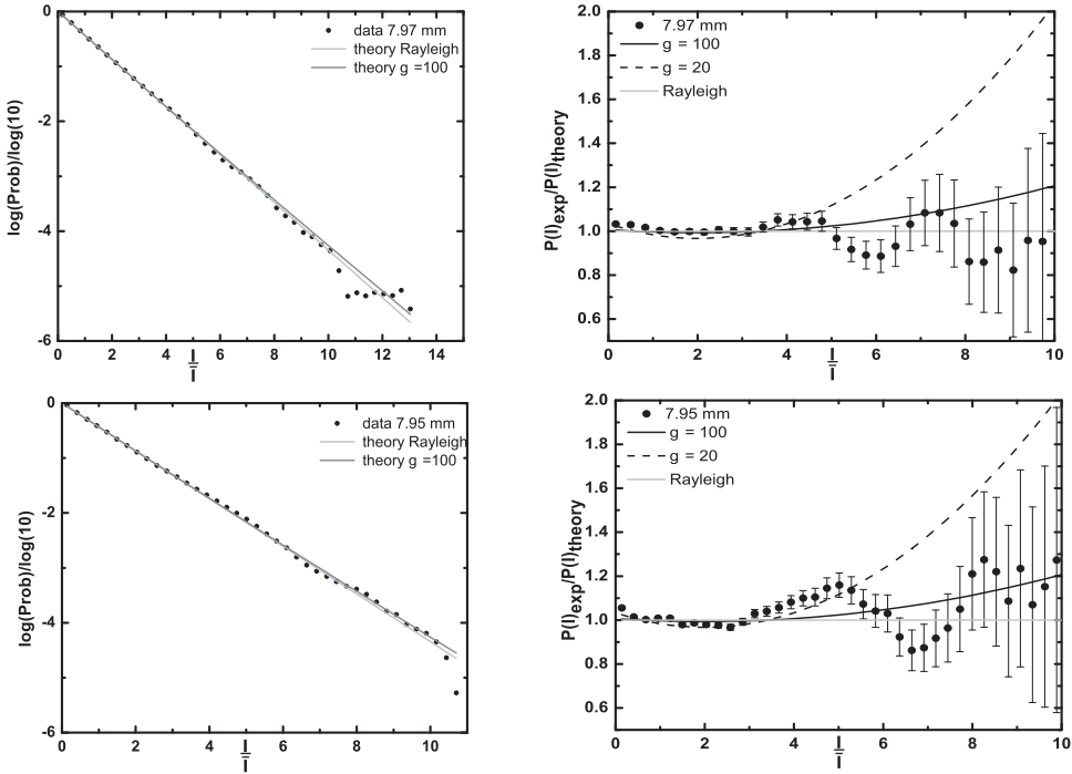
Figure 4.10: (left) Intensity probability distributions extracted from two datasets corresponding to positions 7.97 mm and 7.95 mm. The remaining details of the figure are explained in fig. (4.9).
