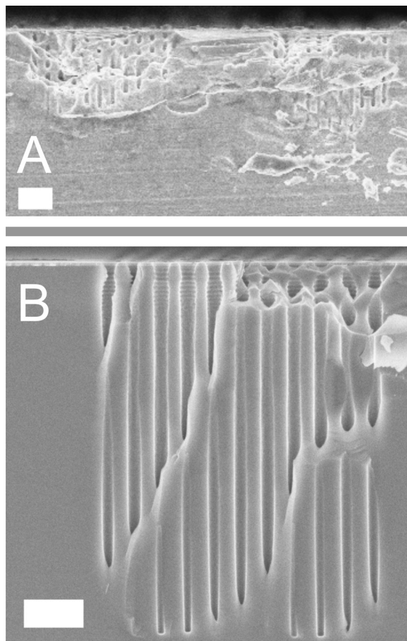
Figure 5.4: A) Scanning electron micrograph of a cross-section of an etched sample diced by a dicing saw. The scale bar equals 2\text{ }\mu\text{m} . Many loose pieces of silicon can be seen, as well as large craters that have been cut out by the saw. Because of these craters, many layers of etched pores are visible. The damage to this cross-section surface is significant. B) Scanning electron micrograph of a cross-section of a cleaved sample. The scale bar equals 1\text{ }\mu\text{m} . The sample is not flat, and multiple layers of etched pores are visible. The cleave is not perpendicular to the wafer surface. A piece of silicon has broken off the upper right section of the structure. Both surfaces are not suitable for etching of the second set of pores.
