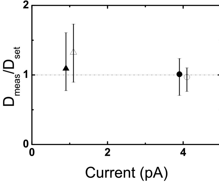
Figure 6.7: Measured cavity size ( D_{\text{meas}} ), relative to the set size ( D_{\text{set}} ) versus milling current. The filled triangles shows the data for colloidal sphere 1 of Figure 6.6, the open triangles show the data for sphere 2, the filled circles are data for sphere 3, and the open circles for sphere 4. The vertical bar through each point depicts the width of the complete white outlining of the cavity on the scanning electron micrograph. The values are slightly offset from 1 and 4 pA for clarity.
