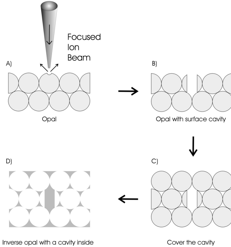
Figure 6.2: : Schematic representation of the fabrication of a nanocavity in an inverse opal. A) Material is milled away with nanometer precision with a focused ion beam. (B) A cavity is achieved in the surface plane of the opal. (C) New layers of colloidal spheres are deposited on top of the crystal to bury the cavity in the bulk. (D). The opal and the embedded cavity are inverted to yield an inverse opal photonic bandgap crystal with a point defect. In this scheme, the cavity is formed by additional high index material that fills the cavity formed by the focused ion beam milling process, thereby creating a donor.
