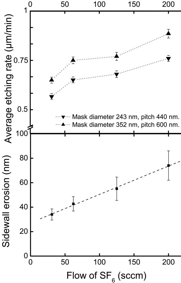
Figure 4.7: A) Average etching rate versus the flow of \text{SF}_6 for two of the diameter-pitch combinations. The average etching rate was calculated by dividing the measured depth of the pores h by the total etching duration. The dotted lines are guides to the eye. B) Sidewall erosion of pores after etching for 6 minutes as a function of the flow of \text{SF}_6 . The sidewall erosion increases with flow.
