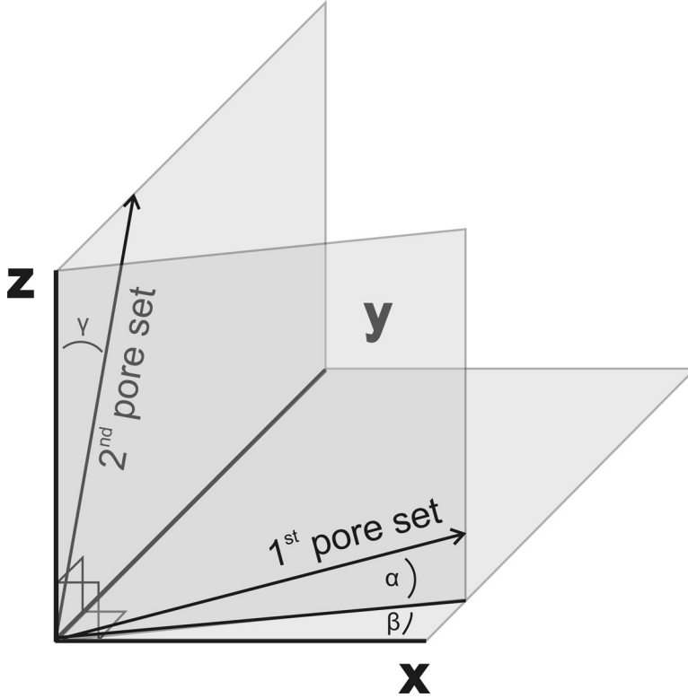
Figure 2.9: Schematic of possible angular misalignments that may occur during the fabrication of a three dimensional photonic structure. The x-axis is the ideal direction of the first pore set and the z-axis of the second pore set. Angular misalignments are introduced when a sample with an existing set of pores is placed in the holder wafer. Misalignment by angle \alpha occurs when the x-axis of the x-y surface of the samples is not mounted parallel to the wafer holder surface. Misalignment by angle \beta occurs when the retrieved sample is mounted in the wafer holder with an in-plane rotational error. Misalignment by angle \gamma occurs when a sample is mounted in the wafer holder with the y-axis of its x-y surface not parallel to the wafer holder surface.
