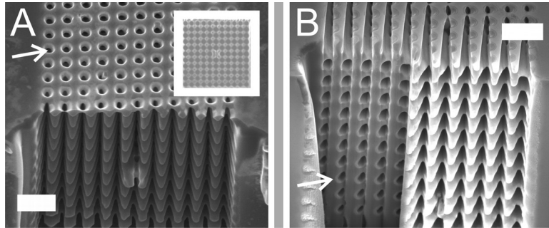
Figure 7.6: Scanning electron micrographs of two three-dimensional monoclinic P photonic crystals, fabricated by i) reactive ion etching and ii) focused ion beam milling. The crystals are observed in a tilted fashion, with at the top the surface of the silicon wafer and below the cleaved cross-section. The scale bars equal 1\text{ }\mu\text{m} . A) The second set of pores was milled exactly through the first. The second pore set can be observed as dark windows penetrating the pore walls of the etched pores, see arrow. The crystal extends over many layers. One pore is not milled, to create a line-defect in the three-dimensional crystal. The inset shows a view parallel to the milled pores. The line defect is visible in the middle of the milled area. B) A crystal without line-defect. Part of the milled crystal was polished away to observe the inside. When going from the top-surface to deeper inside the crystal, the diameter of the pores is reduced due to redeposition of silicon. Redeposited silicon is visible as a lighter shade of grey on the edges of the milled pores, see arrow.
