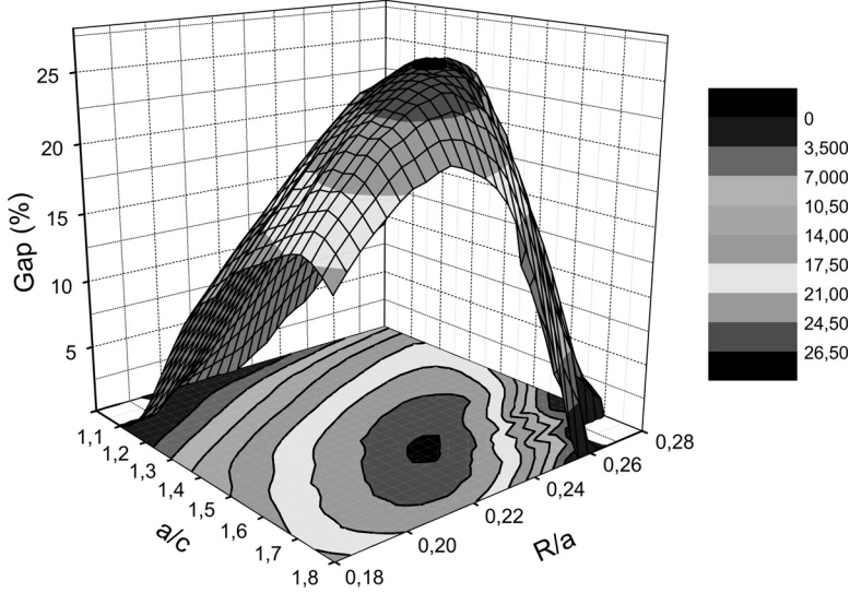
Figure 2.15: Interpolated three-dimensional surface- and contour plot of the calculated band gaps versus the ratios (R/a) and (a/c) . The Figure shows that there is a large region of (a/c) and (R/a) combinations where the relative width of the band gap is much larger than (\Delta\omega/\omega) = 26.5\% , see the black circular area around (a/c) = 1.6 and (R/a) = 0.23 . The broadest photonic band gap of (\Delta\omega/\omega) = 26.9\% is found at (a/c) = 1.575 and (R/a) = 0.23 . The Figure also shows that when a three-dimensional crystal is fabricated from two sets of hexagonal cylindrical pores with high symmetry ( a/c = 1 ), there is only a very small band gap found.
