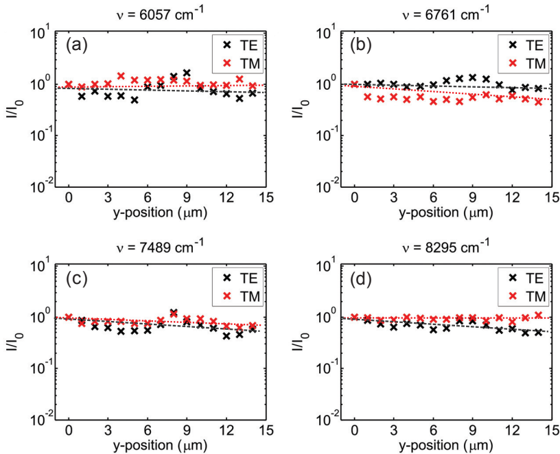
Figure 7.6: Intensity of the out-of-plane scattering of the Teflon sample as function of the lateral y -position of the collecting aperture. (a) though (d) show the intensity distribution for TE (black cross) and TM (red cross) polarized incident light at mean frequencies of \nu=6057 , 6761 , 7489 and 8295\text{ cm}^{-1} respectively. The dashed red and black lines are guides to the eyes.
