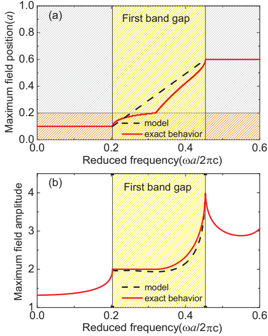
Figure 3.5: (a) Behavior of the first field maximum in the frequency range of the first bandgap. The ordinate between 0 and 0.2 is the high index material (indicated by the orange hatched bar) and from 0.2 to 1 is the low index material (indicated by the gray hatched bar). The red solid line is the exact behavior of the field and the black dashed line is the linear interpolation with the position. (b) Comparison of the exact maximum field amplitude (red curve) and the model (black dashed curve) as a function of reduced frequency. In the model a linear interpolation is used for the position of the field maximum (see(a)). The model shows a very good agreement with the exact calculations.
