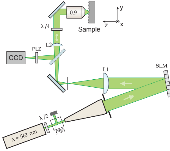
Figure 6.2: Schematic illustration of the wavefront shaping setup. A laser with wavelength \lambda = 561 \text{ nm} is used as light source. The laser beam passes through a half wave plate ( \lambda/2 ) and a polarizer beam splitter ( PBS ) to obtain a known incident polarization. The beam is expanded using a beam expander to cover an area of 8 \text{ mm} by 8 \text{ mm} on the spatial light modulator (SLM). Light that is reflected back from the SLM passes through L1 lens and is spatially filtered using an aperture. The laser light is then focused on the sample surface using a high numerical aperture objective with NA = 0.9 . A camera is in the imaging configuration to image the sample surface. A polarizer and a quarter wave-plate are placed in the reflection path to filter the direct reflection from the sample surface. For alignment purposes a white light source illuminates the sample surface.
