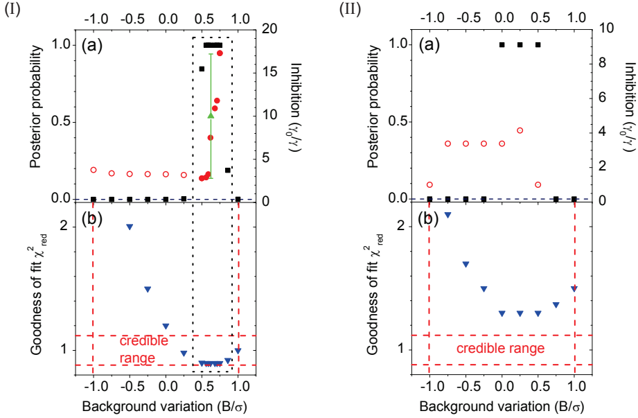
Figure 5.3: Maximum a posteriori estimation analysis of the time-resolved emission of the near-infrared PbS quantum dots in a 3D photonic band gap crystal. I(a) Overall a posteriori probability function P_{max}(B, \{p_i\}|\{y_i\}, N_{bt}) (black squares) versus background parameter B normalized to background standard deviation \sigma for emission data obtained at 0.893 eV. The background is varied within the credible range given by Eq. (5.6). Red circles show the simultaneously resulting inhibition \gamma_0/\gamma (right axis). Red closed circles are credible inhibitions that yield the final result shown as the green triangle with error bars. I(b) Reduced goodness of fit \chi_{red}^2 (blue inverted triangles) versus B . The black dashed rectangle emphasizes the range of B where simultaneously the posterior probability is high and the goodness of fit is within its credible range, thus determining the consistent inhibition range. II(a) Overall a posteriori probability function P_{max}(B, \{p_i\}|\{y_i\}, N_{bt}) (black squares) versus background parameter B/\sigma . The background is varied within the credible range. Red open circles show the simultaneously resulting inhibition \gamma_0/\gamma (right axis). II(b) Reduced goodness of fit \chi_{red}^2 (blue inverted triangles) versus B . Since the minimum of the \chi_{red}^2 is not within its credible range, this data set is inconsistent with the assumptions and thus excluded.
