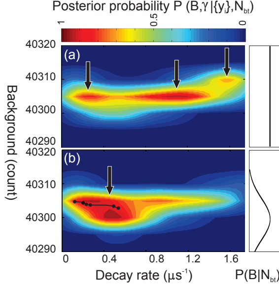
Figure 5.5: Posterior probability distribution plotted for two different prior distributions (Eq. 5.9). (a) Prior distribution is a uniform distribution. Since a uniform distribution is a flat distribution, the posterior distribution in this case is comparable with likelihood of the parameters that in conventional fitting routine would be maximized. The black arrows indicate the high probability regions. (b) Prior distribution is a normal distribution with center of average background value. By applying the normal distribution as prior the posterior distribution has changed and becomes more concentrated in a range of decay rate values. The black circles show maximized posterior probability of decay curve where background is kept fixed.
