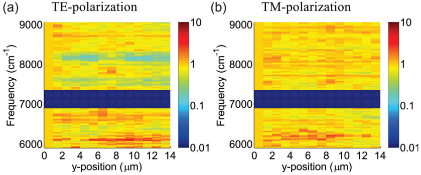
Figure 7.5: Intensity and frequency resolved out-of-plane scattering of the Teflon sample for (a) TE-polarization and (b) TM-polarization. The wide dark blue line is due to the broken diodes in the detection array, corresponding to a frequency of 6900 to 7350 \text{cm}^{-1} . The blue color represents minimum and the red shade stands for maximum intensity of the out-of-plane scattered light. For a direct comparison, the color bar is kept the same as for the measurements on photonic crystals.
