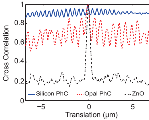
Figure 6.11: One line profile of the cross correlation of the reflected light shown in Fig. 6.10 for opal and silicon crystals, and random scattering sample of ZnO. For both crystals periodicity is seen which matches with the crystal periodicity. The decorrelation in the silicon photonic crystal is only about 0.14, indicating a very good crystal quality. For the opal crystal correlation is to a minimum of around 0.6, which shows contribution of more disorder compared to the silicon crystal. For reference cross correlation of random scattering sample of ZnO is presented, showing a decorrelation of about 0.8.
