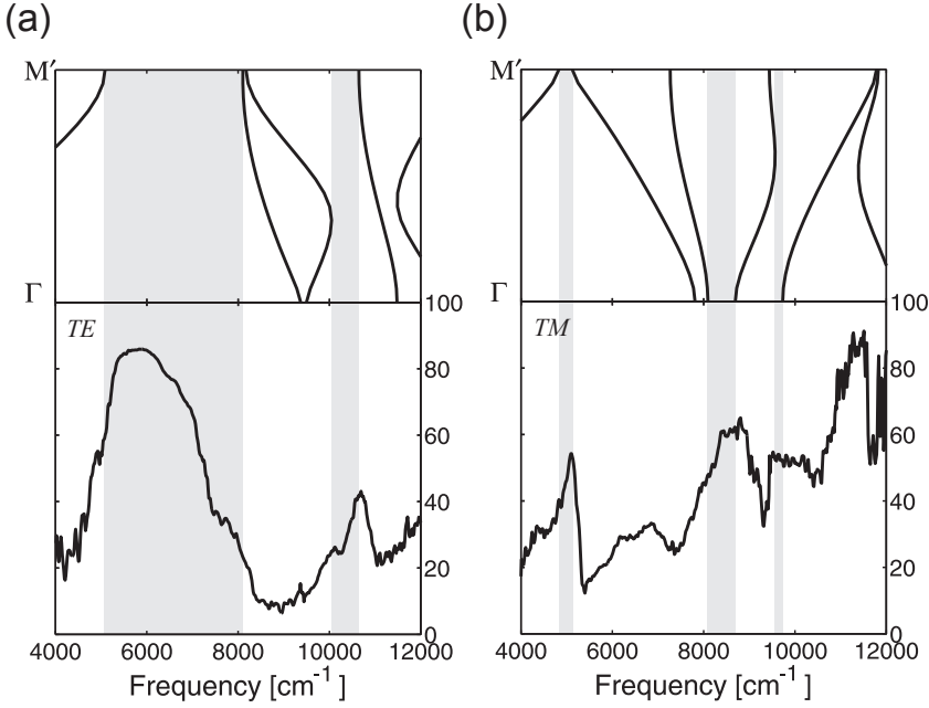
Figure 7.2: Calculated band structure and measured reflectivity of the two-dimensional photonic crystal sample (sample code Ad3c-28112008) as function of frequency for (a) TE and (b) TM polarized light incident along the \Gamma M' direction of the photonic crystal [17]. The gray bars indicate the calculated stop gaps.
