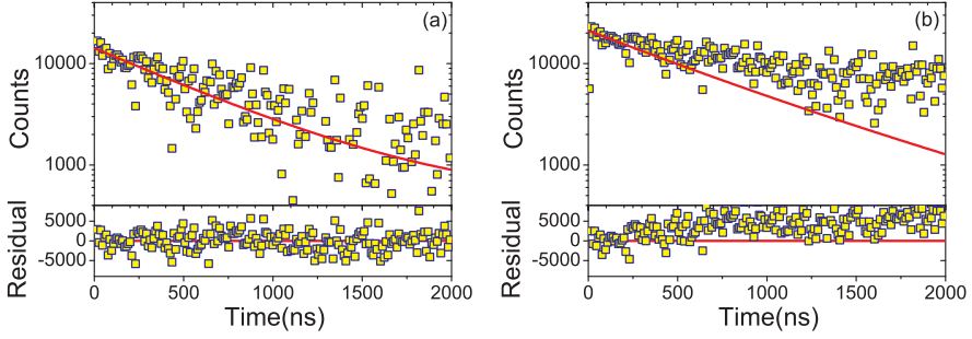
Figure 5.4: comparison of one near infrared data set ( \lambda = 1390nm ) with different background subtraction. (a) Subtracting of (\frac{N_{bt}}{n} + 3\sigma/4) as background yields the best fit with residuals centered around zero and a minimized \chi^2_{red} within credible range. (b) Subtracting of (\frac{N_{bt}}{n} - \sigma/2) as a background yields residuals that are not centered around zero and a \chi^2_{red} outside the credible range.
