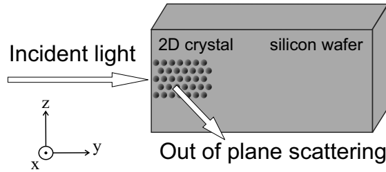
Figure 7.3: Schematic representation of a typical out-of-plane scattering scheme. Incident light illuminates the crystal from the x-z face. In the perpendicular direction the resulting out-of-plane scattering is collected.
