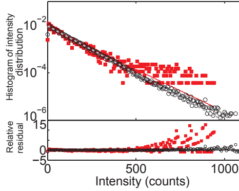
Figure 6.5: Histogram of the intensity distribution from the ZnO (black circles) and opal photonic crystal (red rectangles). The dashed gray line and the solid red line show the Rayleigh statistics and the bottom panel shows the residual; deviation of each distribution from the Rayleigh statistics.
