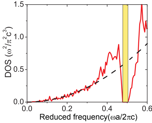
Figure 4.5: Density of states (DOS) per volume for the same crystal shown in Fig. 4.2 calculated with 10000 k points. The DOS vanishes in the band gap indicated with a yellow bar. Dashed curve: quadratic behavior in the low frequency limit.
