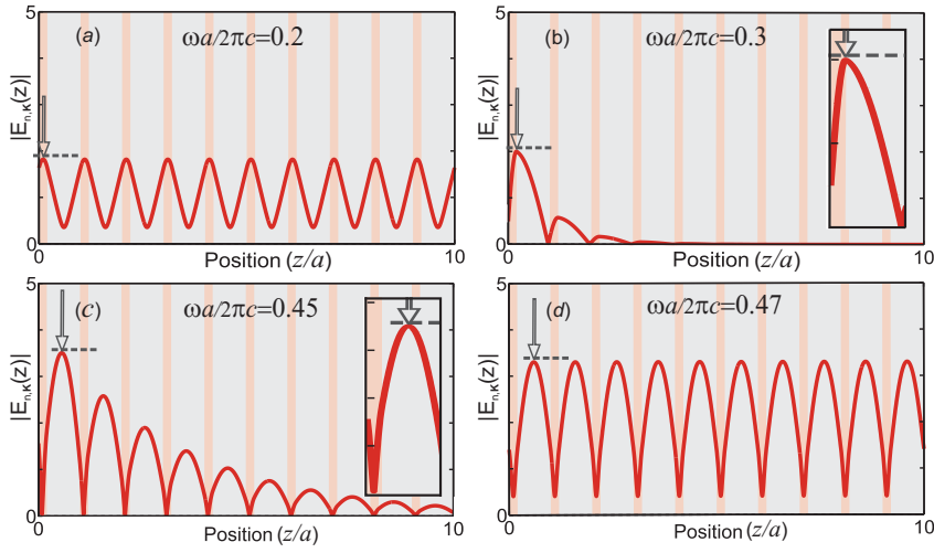
Figure 3.4: Absolute value of the electric field associated with (a) reduced frequency \omega a / 2\pi c = 0.2 , (b) reduced frequency \omega a / 2\pi c = 0.3 , (c) reduced frequency \omega a / 2\pi c = 0.45 , and (d) reduced frequency \omega a / 2\pi c = 0.47 of the band structure plotted in the Fig. 3.3. The main maximum of the field amplitude is indicated in Fig. 3.4 with a black arrow.
