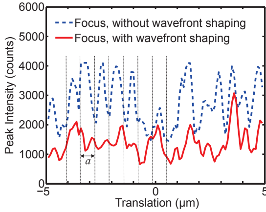
Figure 6.7: The maximum peak intensity of the focus on the sample versus the translation. The translation is over a distance of 10\ \mu\text{m} with steps of 100\ \text{nm} . The blue dashed line is the the maximum focus intensity without wavefront shaping. The unit-cell modulation of the intensity is clearly seen. The red curve is the maximum intensity of the wavefront shaped focus, showing less periodicity.
