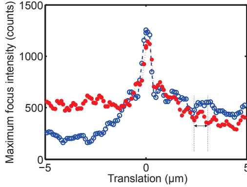
Figure 6.9: Maximum focus intensity for two different wavefront shaping realizations on different positions on the opal crystal. The red curve shows periodicity on both sides, confirming the similarity in the crystal structure over a distance of 10 \mu\text{m} . The periodicity is indicated with a double sided arrow. The blue curve shows periodicity only in one side and a drop in the intensity on the other side. This is probably because on the left side the focus has moved to a different grain.
