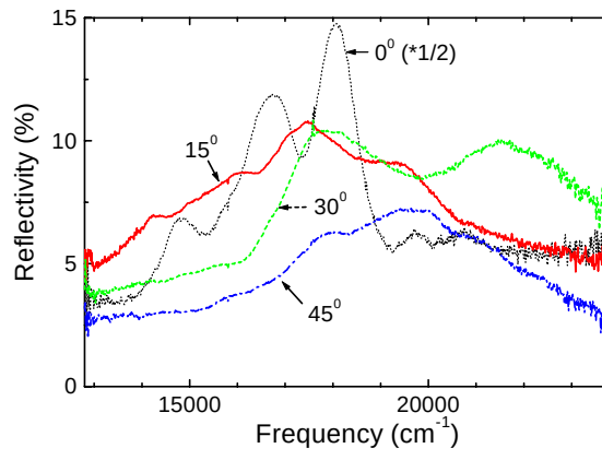
Figure 18: Reflection spectra of titania air-sphere crystals for angles of incidence of \theta (dotted curve, same as in Fig. 17 but multiplied by 0.5), 15^\circ (solid curve), 30^\circ (dashed curve), and 45^\circ (dash-dotted curve). 40
