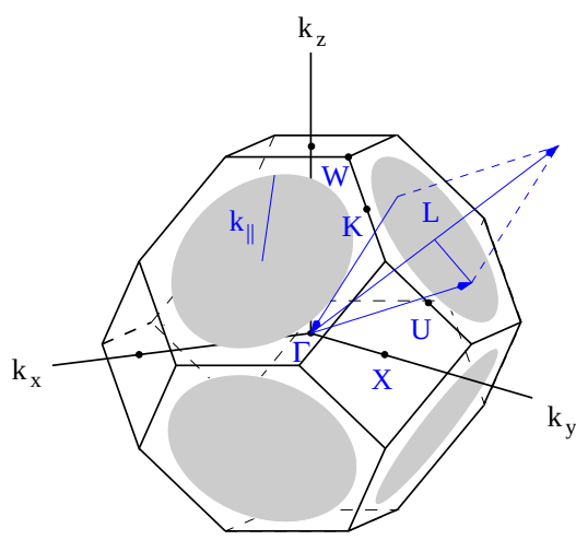
Figure 16: The first Brillouin zone of the fcc structure of the air-sphere crystals. \Gamma indicates the origin of reciprocal space, and K, L, U, and W are high symmetry points on the edge of the Brillouin zone. The arrow from the zone edge to \Gamma denotes the wave vector of an incident light beam, and the arrow from \Gamma to the zone edge indicates the wave vector of a reflected light beam. The long arrow from \Gamma through L is the 111 reciprocal lattice vector that is probed in the experiment. The shaded circles with radius k_{||} = k_L \times 0.59 indicate the range of wave vectors for which light with a frequency at the top of the L-stop band is reflected. 18
