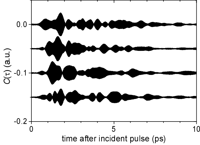
Figure 12. Interferograms from a number of different speckles measured on a sample of A-GaP of L = 15 \mu\text{m} thickness.
