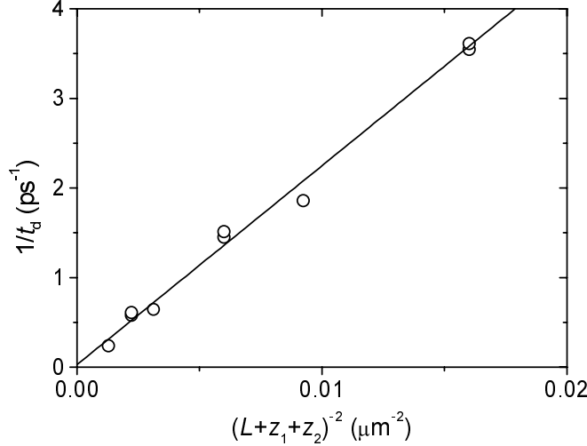
Figure 14. Decay rate of the tail of the transmitted pulse versus the inverse of the thickness squared. The solid line is a linear fit to Eq. 13.
