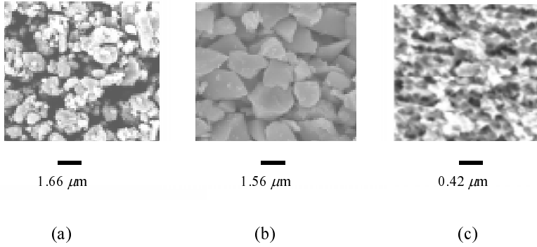
Figure 1. Scanning electron microscope images of disordered semiconductor samples. (a) Si powder, (b) Ge powder and (c) porous GaP (PA-GaP).
