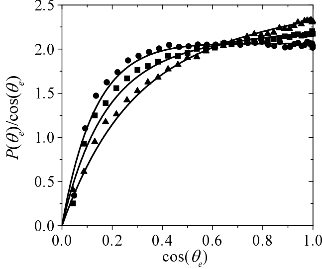
Figure 3. Transmission probability of a PA-GaP as a function of \cos(\theta_e) , where \theta_e is the transmission angle with respect to the sample surface normal. The triangles and circles are the measurements for s and p-polarization detection while the squares correspond to unpolarized detection. The solid lines represent fits to classical diffusion theory from which the effective refractive index of the samples, n_e = 1.5 \pm 0.2 , is obtained.
