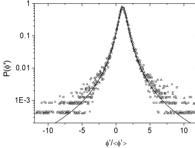
Figure 18. Probability distribution of the phase derivative for sample thickness L = 5 (triangles), 10 (circles), and 18 (squares) \mu\text{m} . The full line is Eq. 18 with Q = 0.4 .
