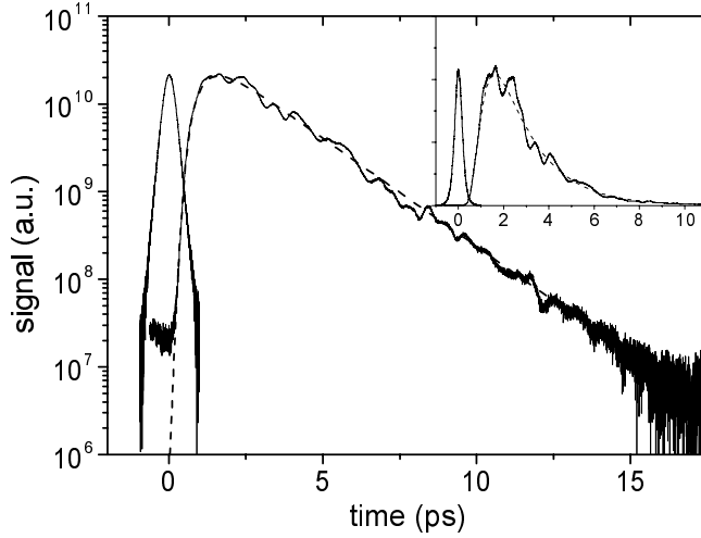
Figure 13. The diffusely transmitted pulse obtained by summing the squares of the interferograms of 60 different speckles of a sample of A-GaP of 15\text{ }\mu\text{m} thickness. The narrow pulse centered around the time origin is the incident pulse. The dashed line is Eq. 12 with D = 21\text{ m}^2/\text{s} and L_a = \infty . Inset: same data on a linear scale.
