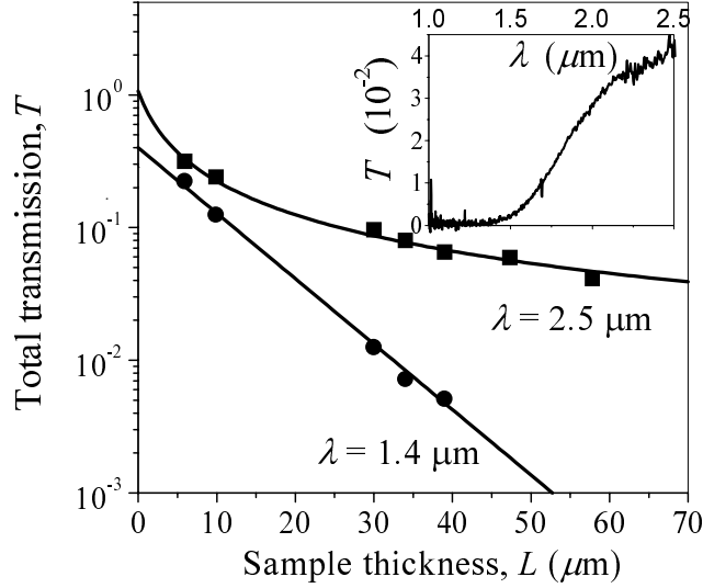
Figure 6. Total transmission through Si powders as a function of the sample thickness, L , for \lambda = 1.4 \mu\text{m} and \lambda = 2.5 \mu\text{m} . The solid lines are fits using classical diffusion theory. The inset shows the total transmission spectrum of a L = 57.8 \mu\text{m} sample.
