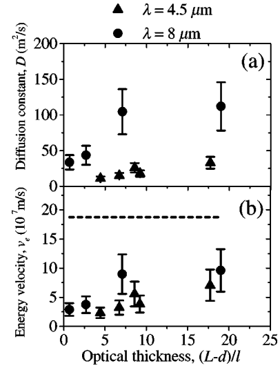
FIG. 13. (a) Diffusion constant D of light at \lambda = 4.5 \mu\text{m} (triangles) and \lambda = 8 \mu\text{m} (circles) in Ge powder samples as a function of the sample optical thickness. (b) Energy transport velocity in the same samples and at the same wavelengths. The straight dashed line is the phase velocity in an homogeneous medium with a refractive index equal to the effective refractive index of the Ge powder samples.
