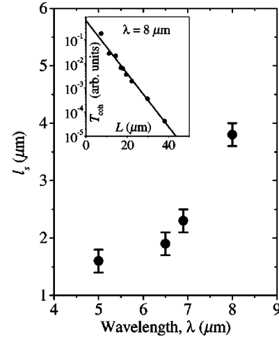
FIG. 4. Scattering mean free path l_s in Ge powder samples as a function of the wavelength, \lambda . Inset: measurements of the transmission of the coherent beam ( \lambda = 8\text{ }\mu\text{m} ) as a function of the sample thickness, L . The line is an exponential fit to the measurements from which we obtain the scattering mean free path l_s . At this particular \lambda , l_s = 3.8 \pm 0.2\text{ }\mu\text{m} .
