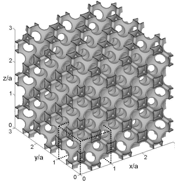
FIGURE 6.3: Model of the inverse-opal structure ( 3 \times 3 \times 3 unit cells): an fcc lattice of air spheres of radius r = 0.25 \sqrt{2}a with a being the cubic lattice parameter. The spheres are covered by shells with \epsilon = 6.5 and outer radius 1.09r . Neighboring air spheres are connected by windows of radius 0.4r . The black cleaved edges are (100) facets. The dashed lines indicate the boundaries of a cubic unit cell.
