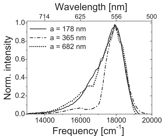
FIGURE 7.1: Normalized emission spectra of R6G in polystyrene opals with three different lattice parameters: a = 178 nm (solid curve), a = 365 nm (dash-dotted curve) and a = 682 nm (dotted curve). In the opal with a = 178 nm, the frequencies of R6G emission lie far below the first-order stopband. Emission from the opal with a = 365 nm reveals the first-order stopband, whose angle-dependence is presented in Chapter 4. Spectrum from the opal with a = 682 nm shows effects of the second-order Bragg diffraction that presented in more detail in Ref. [15].
