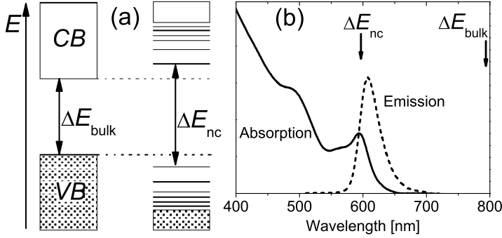
FIGURE 3.8: (a) Schematic band structure of a bulk semiconductor ( left ) and of a nanocrystal ( right ). In the bulk crystal, the energy gap \Delta E_{bulk} separates the populated valence band (VB) from the empty conduction band. In the nanocrystal, the energy-level scheme is discrete; the highest occupied and lowest empty levels are separated by the size-dependent gap \Delta E_{nc} . (b) Measured absorption (solid curve) and emission (dashed curve) spectra of CdSe-ZnSe core-shell quantum dots with the average diameter of 4.5 nm. The emission is measured at a non-resonant excitation with \lambda = 450 nm. The inhomogeneous broadening of the absorption and emission peaks as well as the Stokes shift between the peaks are due to a size dispersion of the nanocrystals [70]. Image courtesy of F. van Driel.
