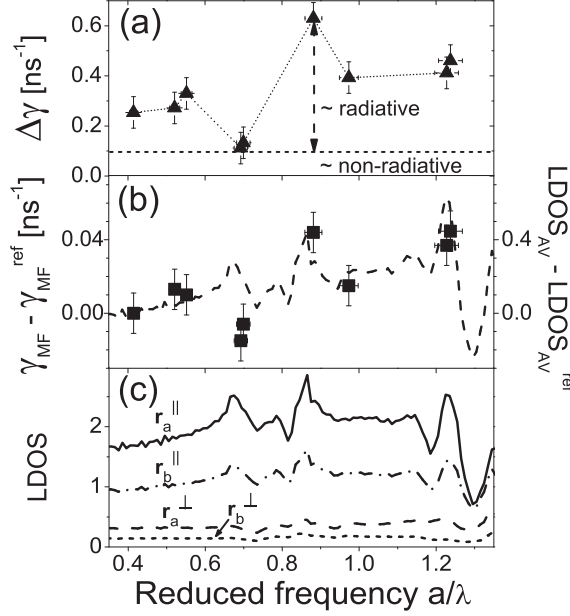
FIGURE 5.5: (a) Width of the decay-rate distribution \Delta\gamma vs. lattice parameter at fixed emission wavelength (triangles, dashed curve is guide to the eye). (b) Difference between \gamma_{\text{MF}} measured on a photonic sample and \gamma_{\text{MF}}^{\text{ref}} = 0.05 \text{ ns}^{-1} of the low-frequency reference (squares). Error bars are estimated from the largest difference between data on samples with similar a . Dashed curve represents the difference between the averaged LDOS in the inverse opals [31] and the averaged LDOS for the low-frequency reference ( \text{LDOS}^{\text{ref}} \approx 0.7 at a/\lambda \approx 0.41 ). The averaging was performed over all dipole orientations and over five points on the internal \text{TiO}_2 -air interfaces: at points a , b , c , d (shown in Fig. 6.5) and \mathbf{r} = (0.23, 0.23, 0.14) . (c) LDOS at two positions on the internal \text{TiO}_2 -air surfaces projected on dipole orientations parallel ( \parallel ) or normal ( \perp ) to the internal surface: at \mathbf{r}_a = \frac{1}{4\sqrt{3}}(1, 1, 2) and at \mathbf{r}_b = \frac{1}{2\sqrt{6}}(1, 1, 1) .
