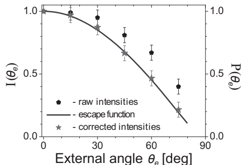
FIGURE 4.4: Angular distribution of the R6G emission from a polystyrene opal with a lattice parameter a = 178 nm. The pentagons indicate the intensity measured at the spectral maximum ( \omega = 17860 cm ^{-1} or \lambda = 560 nm), the solid curve is the calculated escape function with Fresnel internal-reflection coefficient. Measured intensities corrected for the detection efficiency of the set-up are displayed as stars. All data are normalized at \theta_e = 0^\circ .
