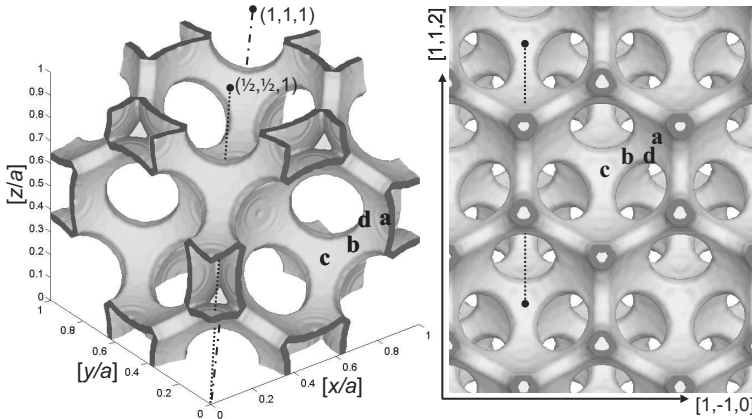
FIGURE 6.5: (Left) View of a single unit cell of the modeled inverse opal. (Right) Cut of the inverse opal along (111) facet. The letters indicate different positions at the \text{TiO}_2 -air interface equivalent to: \mathbf{a} = \frac{1}{2\sqrt{2}}(1,0,0) , \mathbf{b} = \frac{1}{4\sqrt{3}}(1,1,2) , \mathbf{c} = \frac{1}{2\sqrt{6}}(1,1,1) and \mathbf{d} = (0.33, 0.13, 0) . The dash-dotted line (Left) shows the main diagonal of the cubic unit cell. The dotted line (Left and Right) indicates [1,1,2] direction that belongs to the (111) crystal plane.
