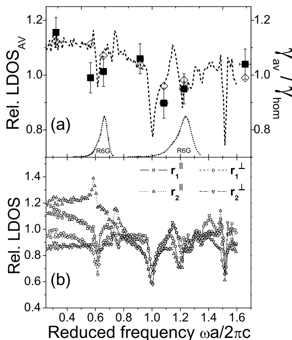
FIGURE 7.4: (a) Decay rates of R6G (squares) measured at \omega = 17985 \text{ cm}^{-1} and normalized to the rate in a homogeneous medium \gamma_{hom} = 0.254 \text{ ns}^{-1} . Dipole- and position-averaged relative LDOS (dashed curve). The averaging was performed over five points on the internal surfaces: at \mathbf{r}_1 = \frac{1}{2\sqrt{2}}(1,0,0) , \mathbf{r}_2 = \frac{1}{2\sqrt{6}}(1,1,1) , \mathbf{r}_3 = \frac{1}{4\sqrt{3}}(1,1,2) , \mathbf{r}_4 = (0.33,0.13,0) and \mathbf{r}_5 = (0.23,0.23,0.14) . Normalized rates (diamonds) calculated from the averaged LDOS using Eq. 7.4. Dotted curves indicate R6G emission spectrum plotted vs. reduced frequency for in opals with a = 365 and 682 \text{ nm} . (b) Relative LDOS at two positions on internal opal surfaces, \mathbf{r}_1 and \mathbf{r}_2 , projected on dipole orientations parallel ( \parallel ) or normal ( \perp ) to internal polystyrene-air interfaces.
