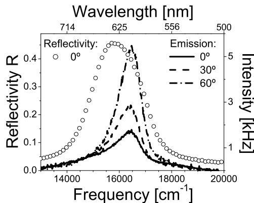
FIGURE 4.7: Normal-incidence reflectivity spectrum (circles) and emission spectra of CdSe quantum dots (curves) in a titania inverse opal with a lattice parameter a = 420 nm. The emission spectra are measured at \theta_e = 0^\circ , 30^\circ and 60^\circ (shown by the solid, dashed and dash-dotted curves, respectively).
