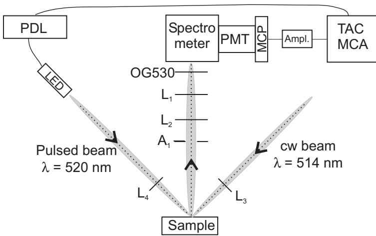
FIGURE 6.2: Schematic of optical set-up used for lifetime measurements. The pump beam, a pulsed LED ( \lambda = 520 nm), is focussed via L_4 on the (111) surface of the sample. The cw beam is needed for bleaching the surface before performing lifetime measurements. The fluorescence of the excited light is collected in reflection. The photons are detected with a MCP via a PMT which is protected against direct reflected light with a Schott OG530 cut-off filter. The MCP signal is amplified and together with PDL signal fed to a TAC and MCA, which records the time difference between the signal and the excitation pulse.
