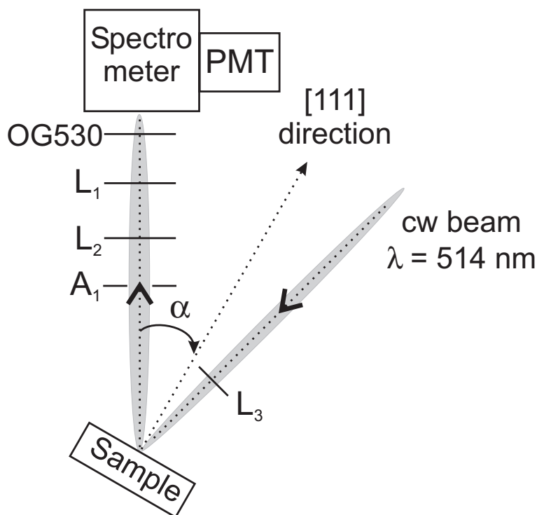
FIGURE 5.3: Schematic of optical set-up. The pump beam of an Argon laser ( \lambda = 514 \text{ nm} ), is focussed on the (111) surface of the sample. The fluorecence of the excited light is collected in reflection with an angle \alpha away from the surface normal. Lens L_3 focuses the laser beam before it hits the sample, L_1 collimates and L_2 focuses the emitted light before it reaches the spectrometer. With aperture A_1 the angular spread of the emitted light can be adjusted. The photons are detected with a photomultiplier tube (PMT) via a prism spectrometer. The PMT is protected against direct reflected laser light by an OG530 cut-off filter.
