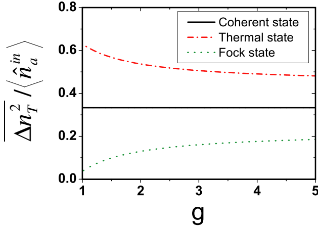
FIG. 4 (color online). Fluctuations of the total transmission for a coherent state, a thermal state with \langle \hat{n}_a^{\text{in}} \rangle = 1 , and an arbitrary Fock state as a function of the mesoscopic conductance g and for a fixed amount of disorder: \ell/L = 1/3 . For decreasing g , the mesoscopic correlations either enhance or suppress quantum fluctuations for the thermal state and the Fock state, respectively. The fluctuations of the coherent state are unaltered for all values of g . When g approaches unity, the localization regime is entered and the model is invalid.
